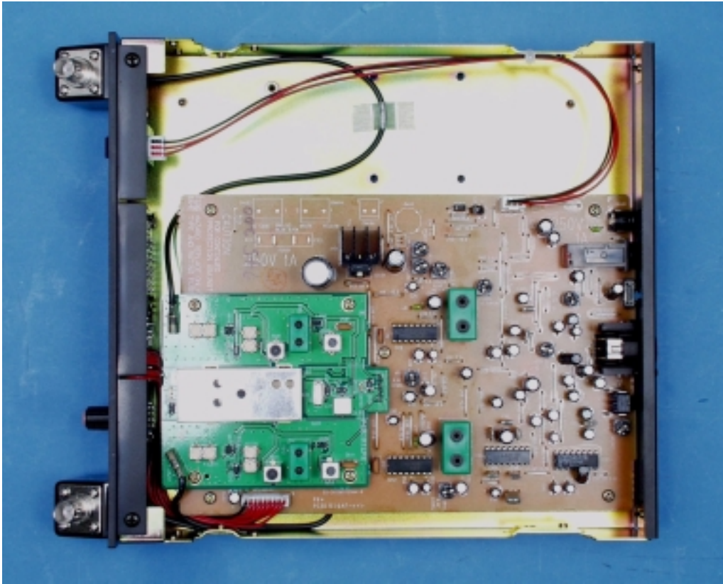
Interior Top View
