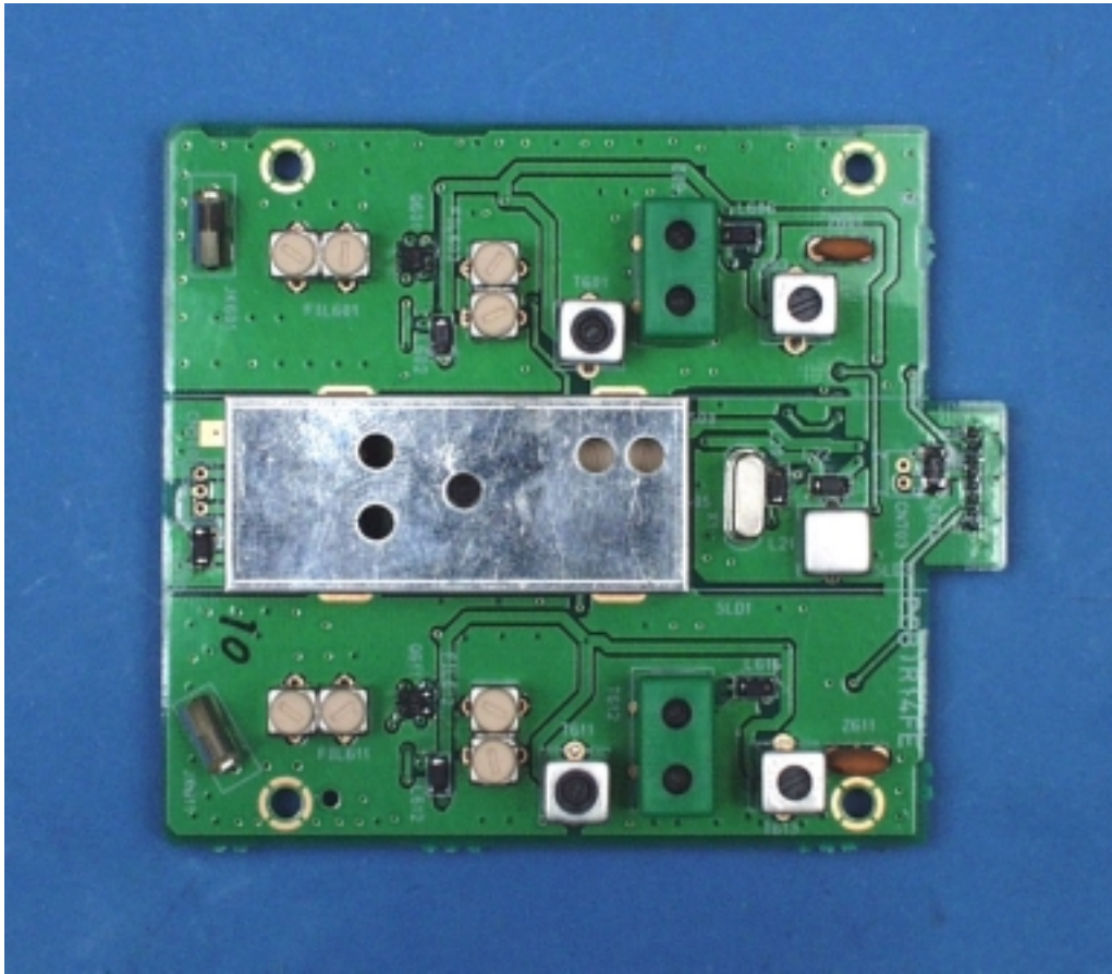
RF Board Top
