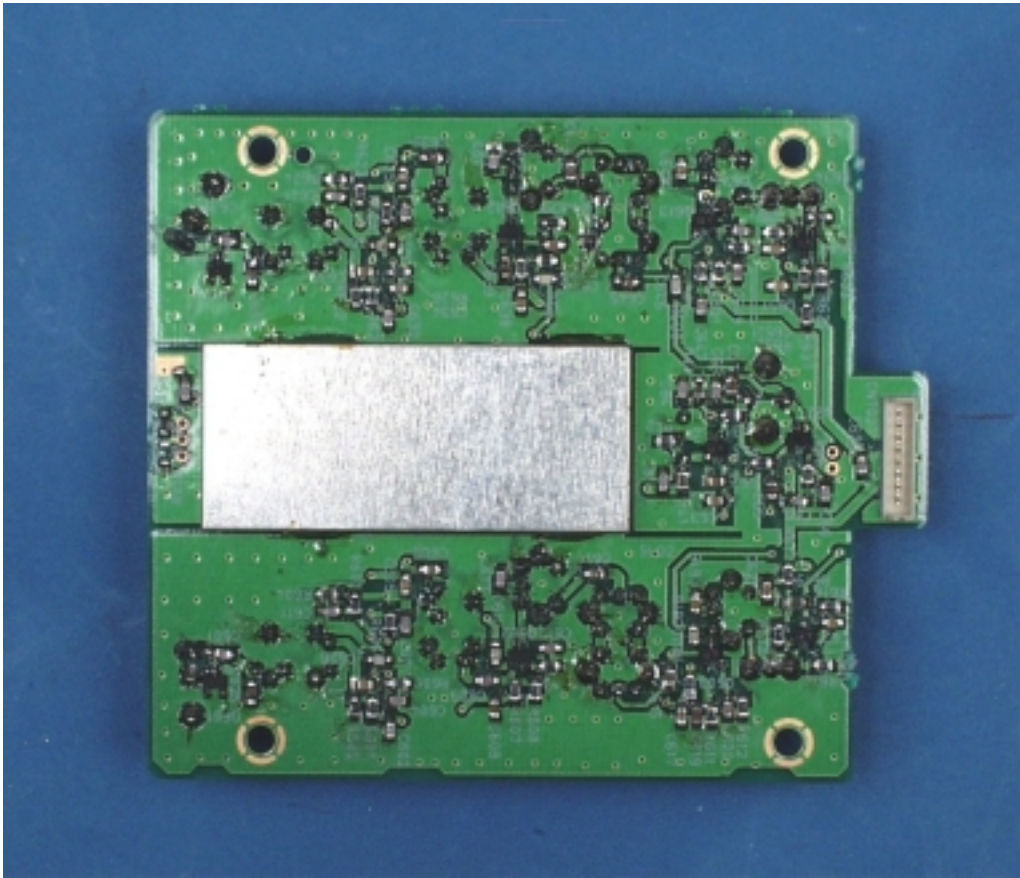
RF Board Bottom
