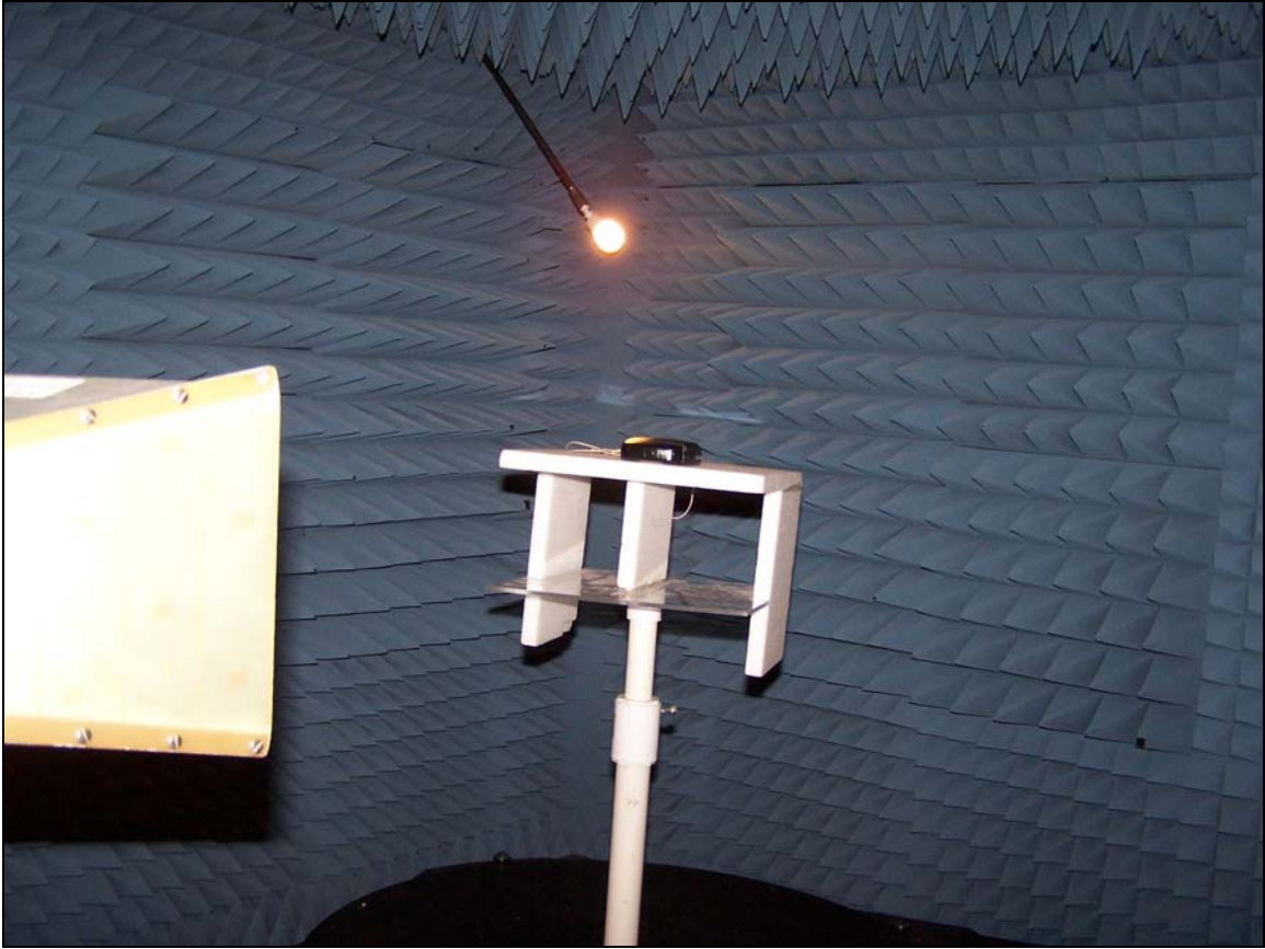
Photograph 7. Spurs above 960 MHz
