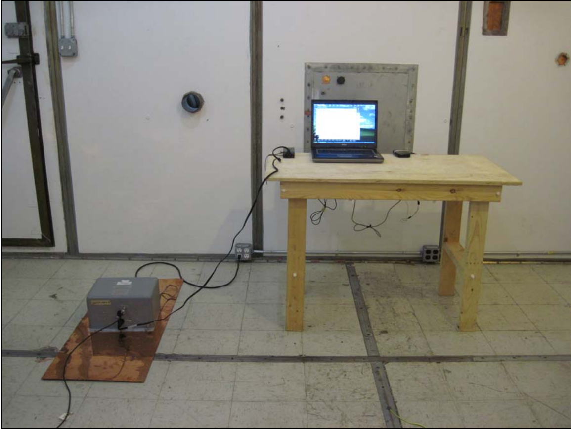
Photograph 2. Conducted Emissions, Peripheral Mode
