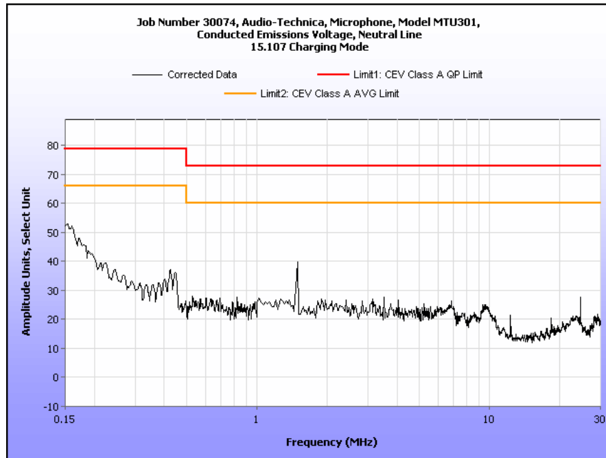
Plot 4. Conducted Emission, Neutral Line Plot, 0.15 MHz to 30 MHz, Charging Mode
