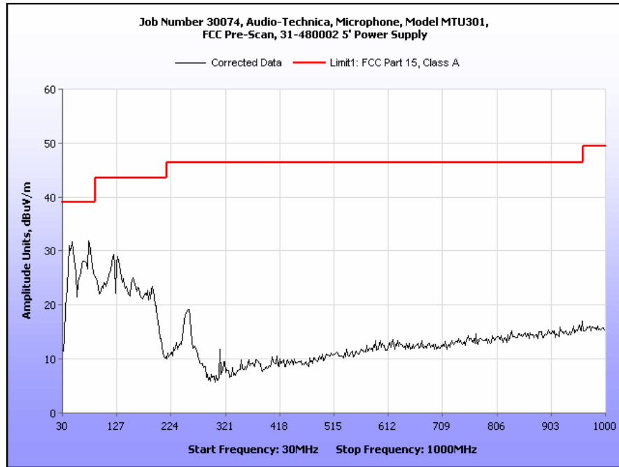
Plot 6. Radiated Emissions, Pre-Scan, Charging Mode
