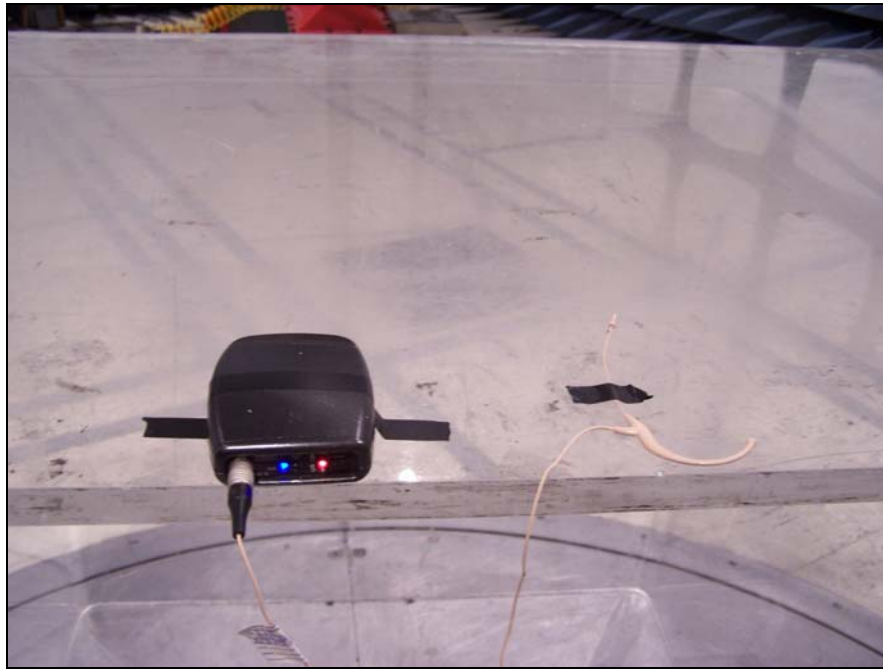
Photograph 3. Radiated Emissions, Test Setup, Running on Batteries
