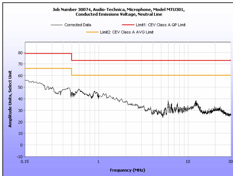
Plot 2. Conducted Emission, Neutral Line Plot, 0.15 MHz to 30 MHz, Class A Computer Peripheral
