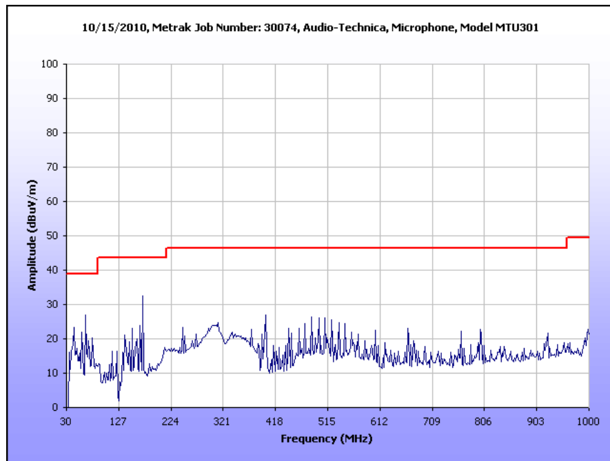
Plot 7. Radiated Emissions, Pre-Scan, Class A Computer Peripheral
