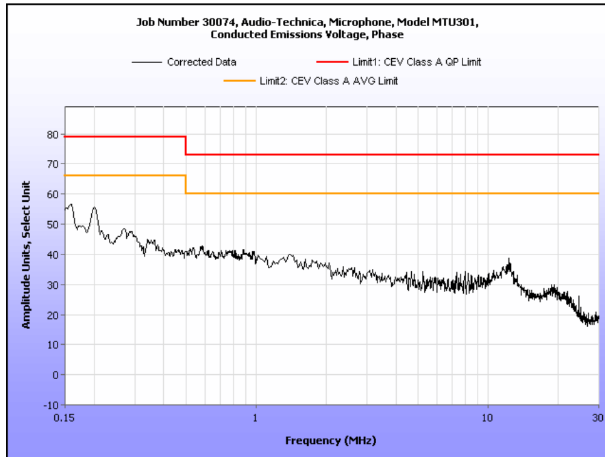
Plot 1. Conducted Emission, Phase Line Plot, 0.15 MHz to 30 MHz, Class A Computer Peripheral
