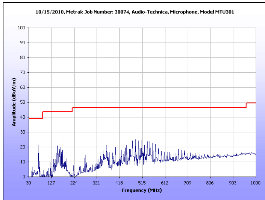
Plot 5. Radiated Emissions, Pre-Scan, Running on Batteries
