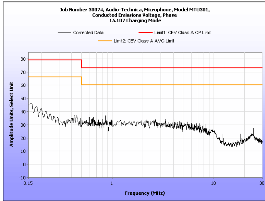
Plot 3. Conducted Emission, Phase Line Plot, 0.15 MHz to 30 MHz, Charging Mode
