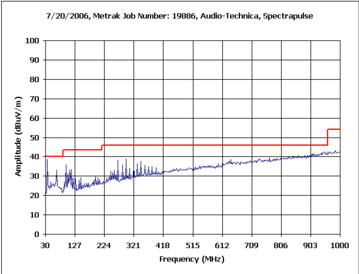
Figure 3. Radiated Emissions Prescan
