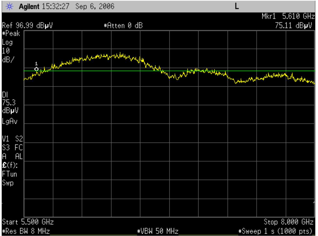
Figure 5. UWB Bandwidth, f_L = 5.610 GHz
