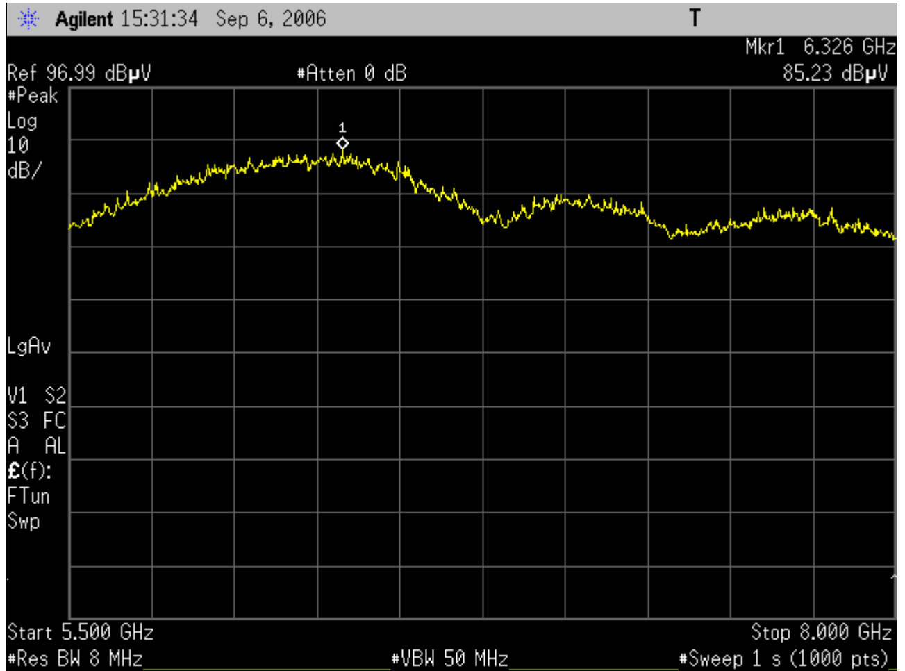
Figure 4. UWB Bandwidth, f_M = 6.326 GHz
