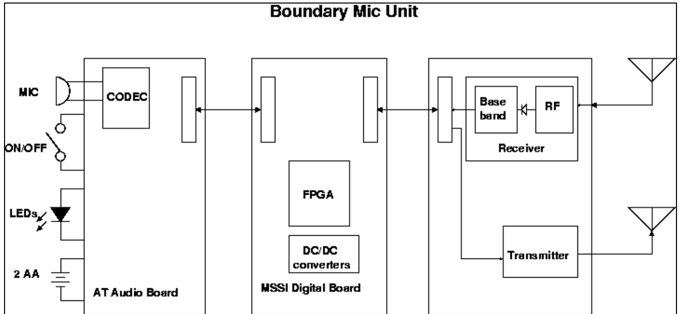
Figure 1. Block Diagram of EUT
