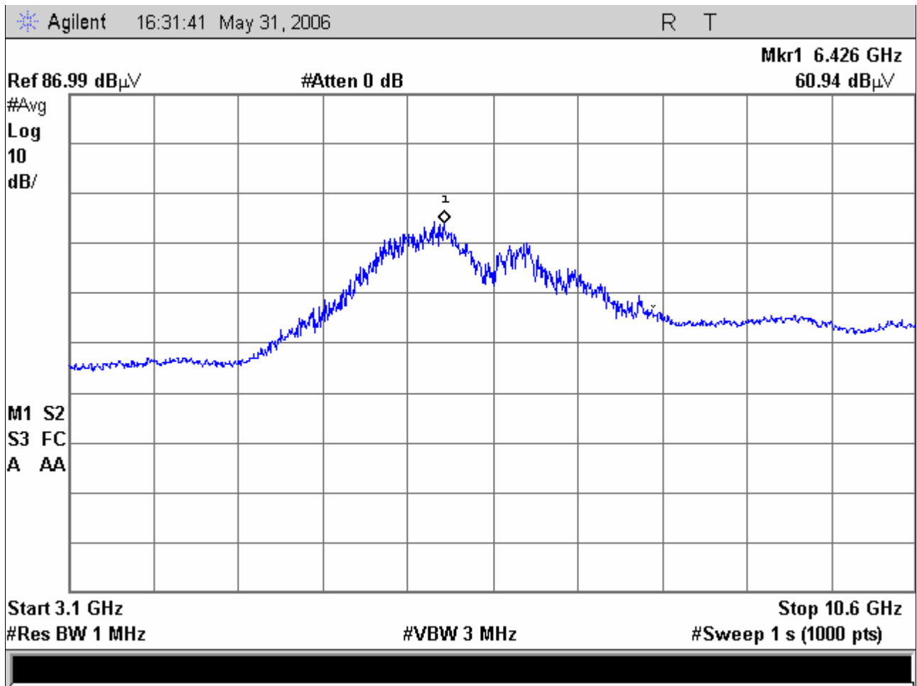
Figure 7. Radiated Emission Limits Test Results, 3.1 GHz – 10.6 GHz
