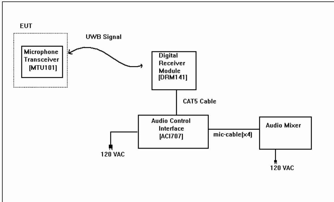
Figure 2. Block Diagram of Test Configuration
