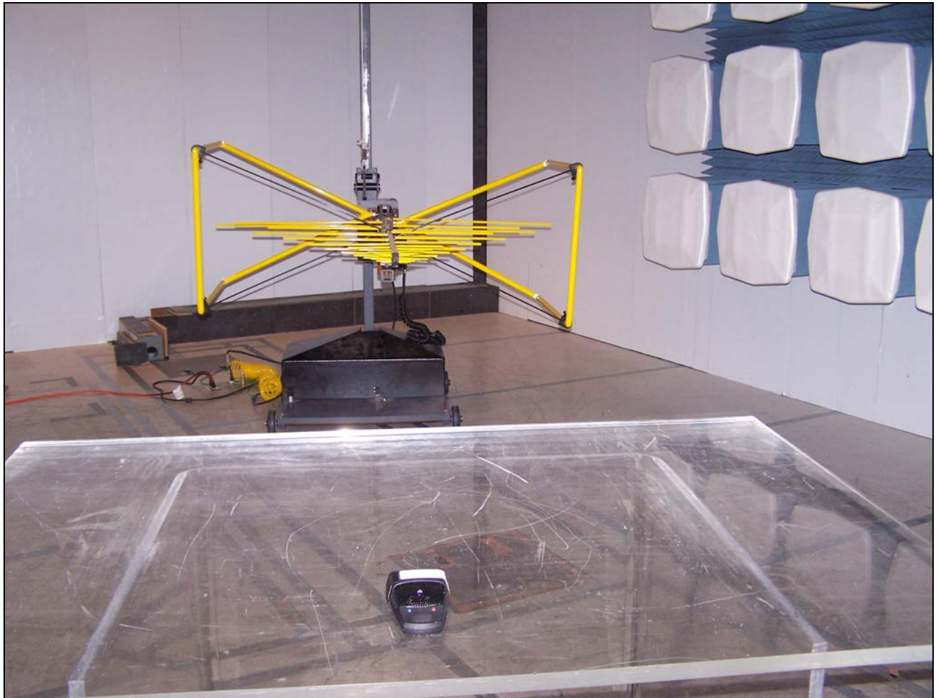
Photograph 3. Radiated Emission Test Setup – 30 MHz to 1 GHz
