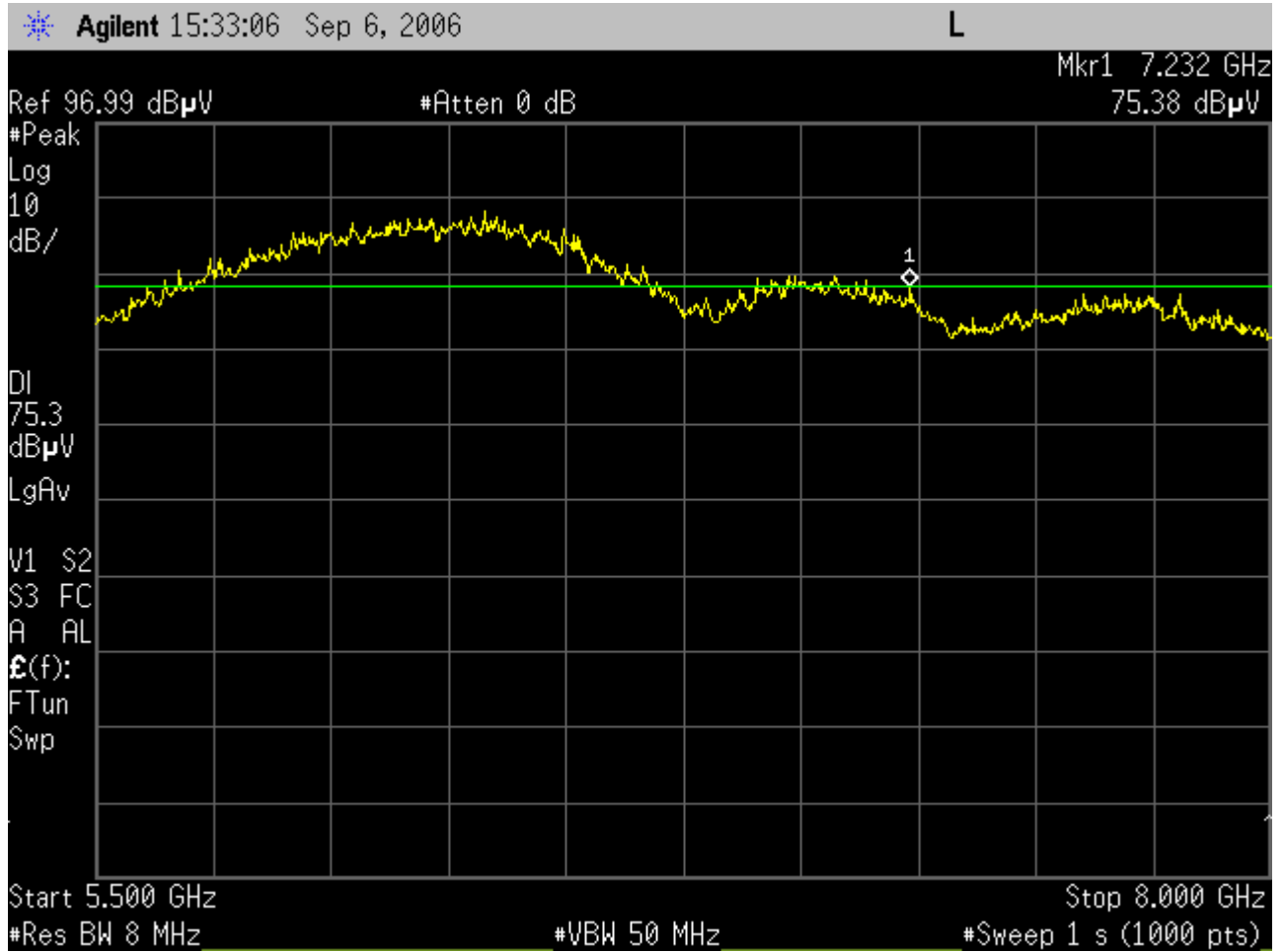
Figure 6. UWB Bandwidth, f_H = 7.232 GHz
