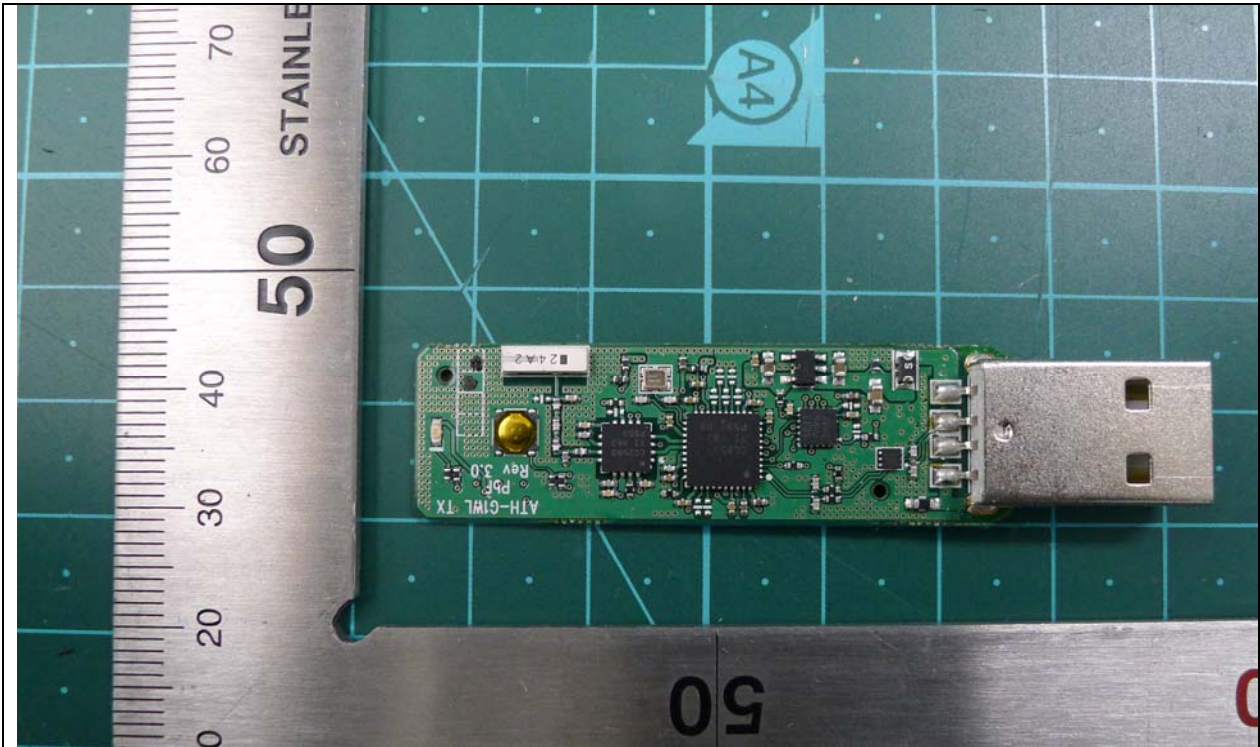
PCB Front
