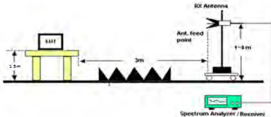
Radiated Measurement
