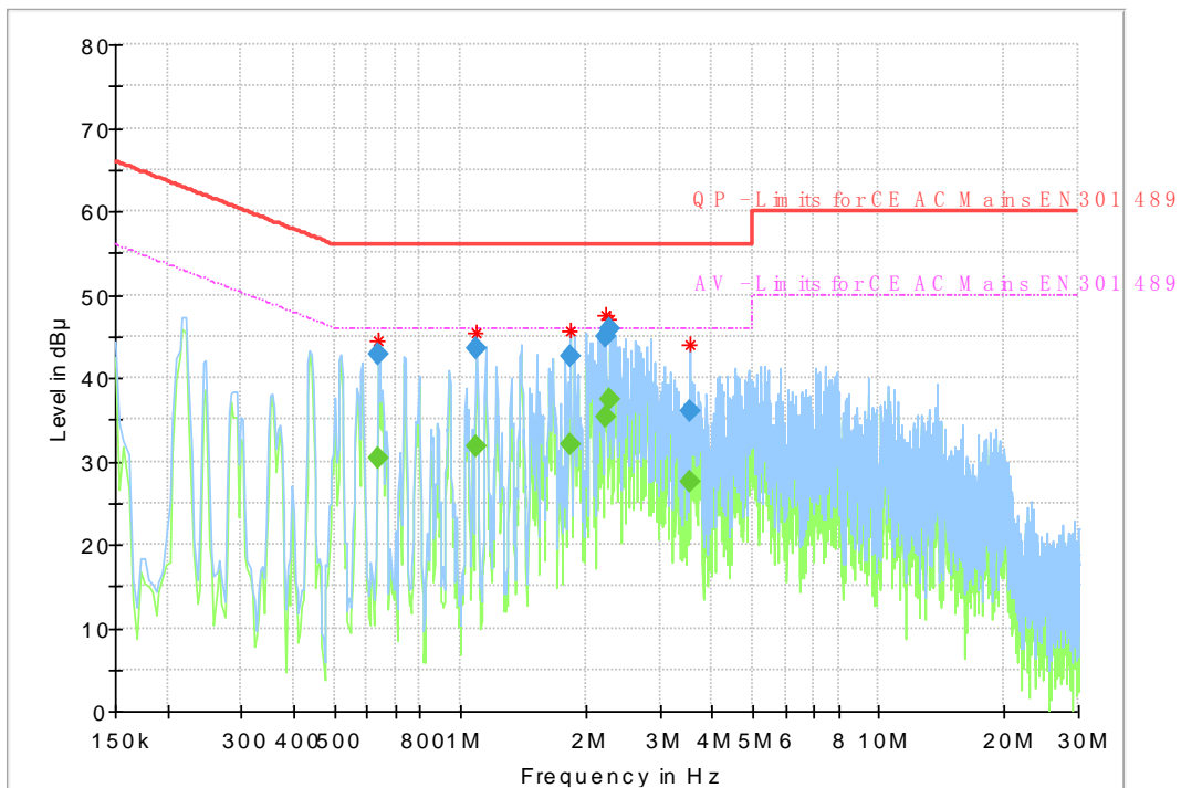
Fig.94 AC Powerline Conducted Emission
