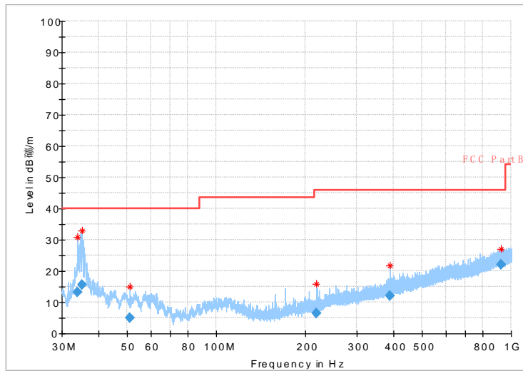
Fig.46 Radiated emission: \pi/4 DQPSK, Ch0, 30MHz~1GHz
