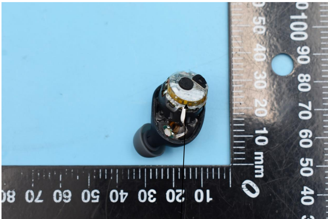
BT Antenna
