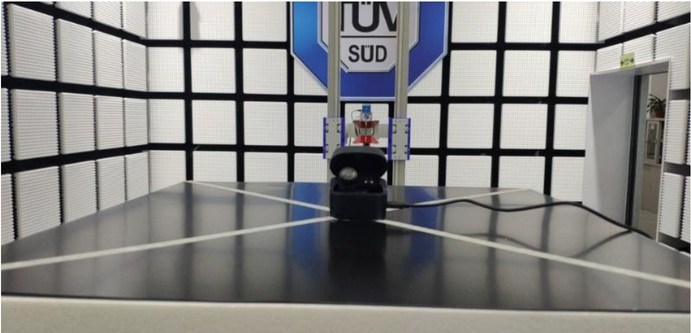
Radiated Emission Test 1GHz-18GHz
