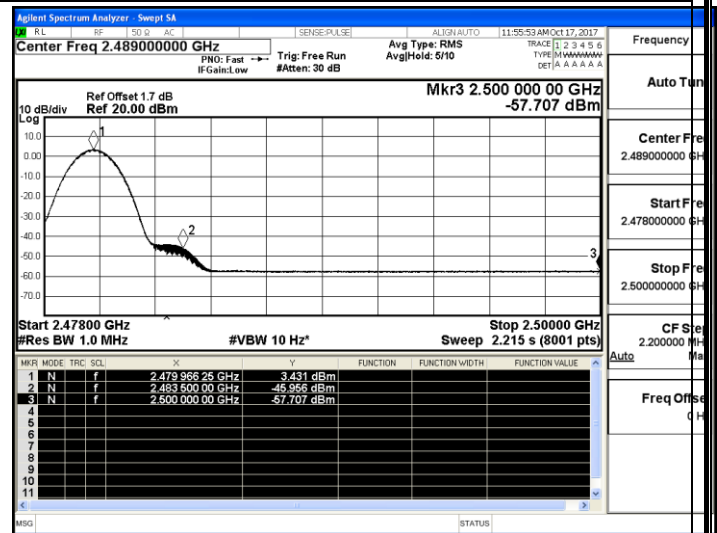
Channel 39 / 2480 MHz – Average
