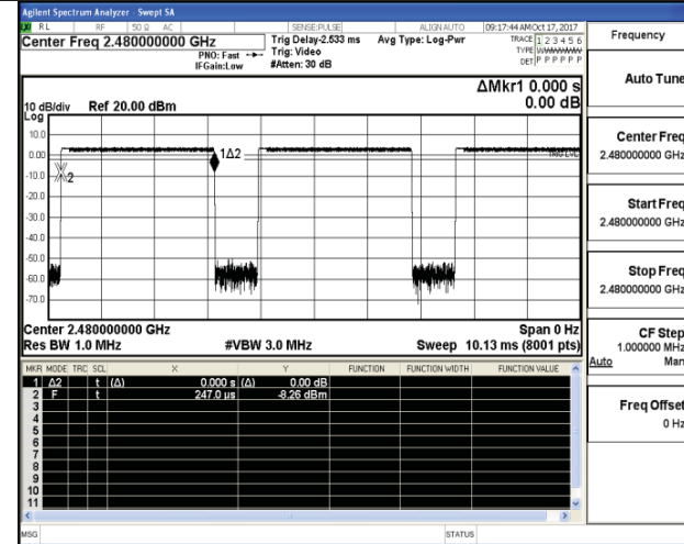
Channel 39 / 2480 MHz - 3DH5
