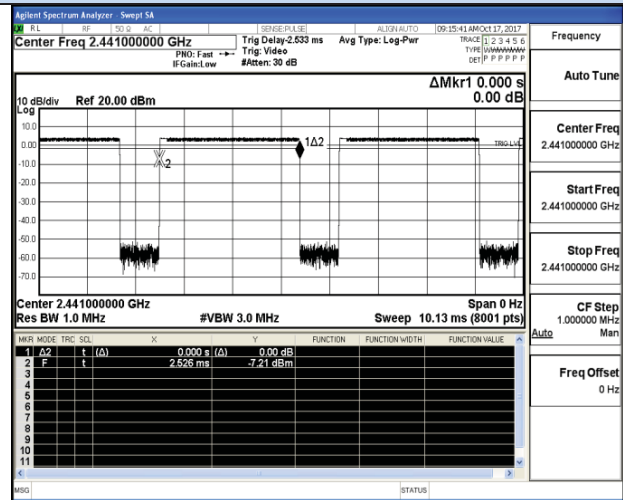
Channel 39 / 2441 MHz - 3DH5
