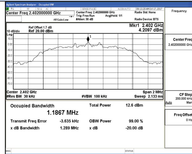
Channel 0 / 2402 MHz
