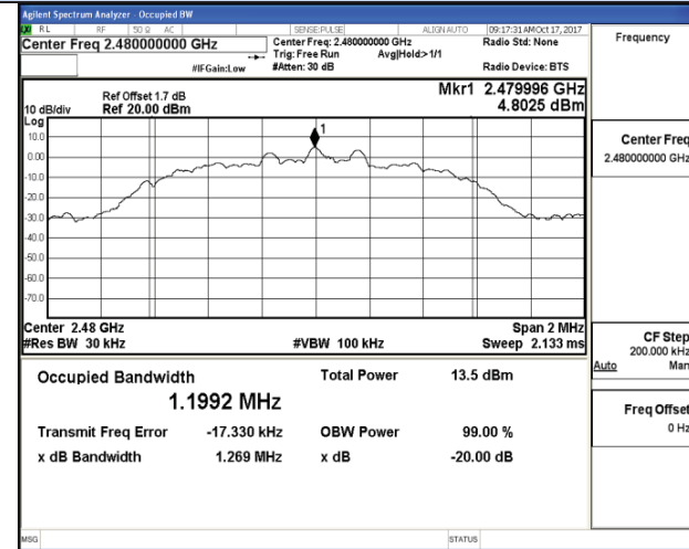
Channel 78 / 2480 MHz
