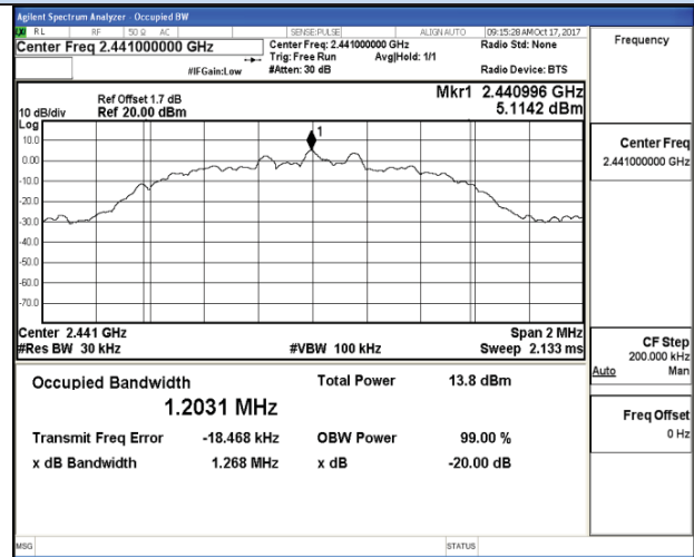
Channel 39 / 2441 MHz
