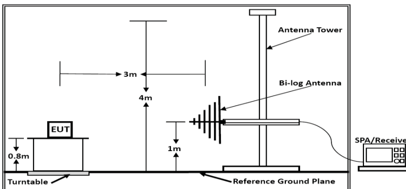
Below 1GHz
