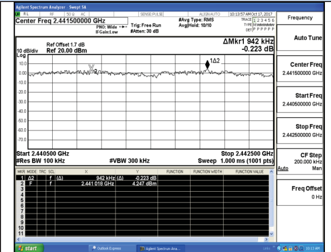
Channel 39 / 2441 MHz
