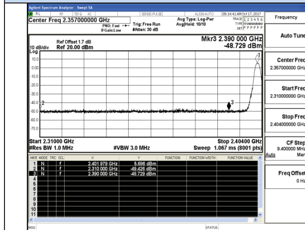
Channel 0 / 2402 MHz –Peak
