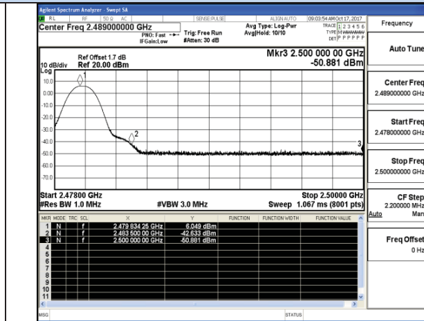
Channel 78 / 2480 MHz –Peak
