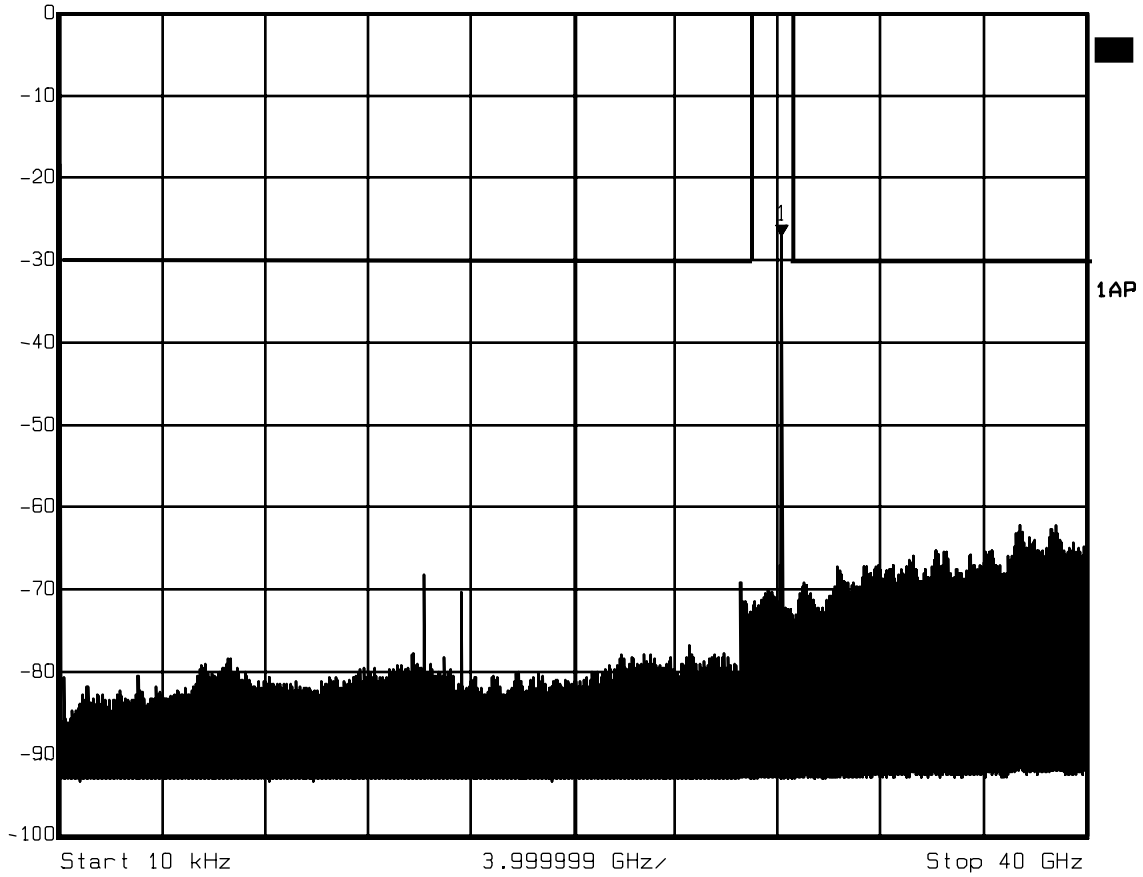
Exhibit 4 - Emissions at the Antenna Port
