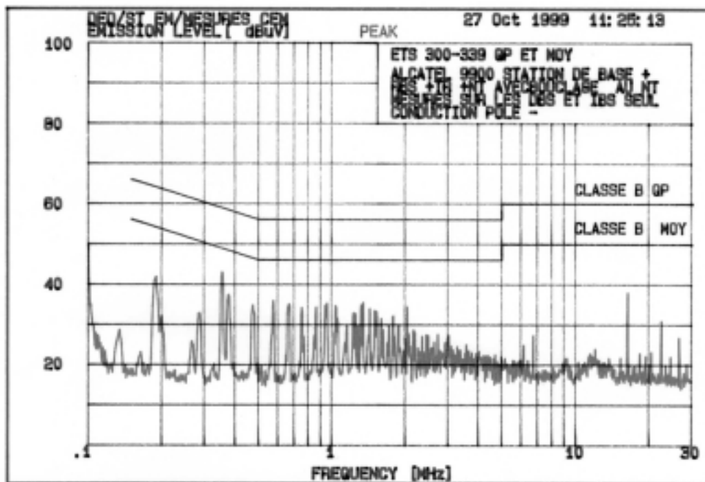
Exhibit 10 - Conducted Emissions on Negative Conductor
