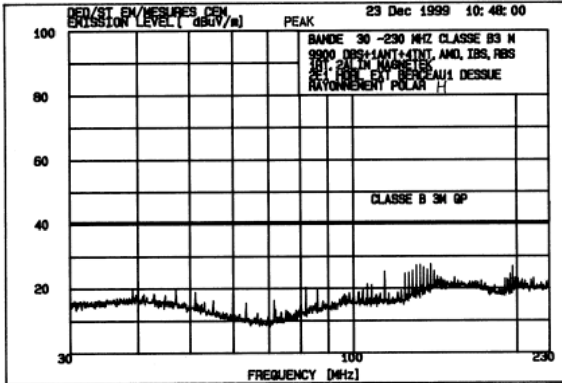
Exhibit 5 - Spurious Radiation (horizontal)
