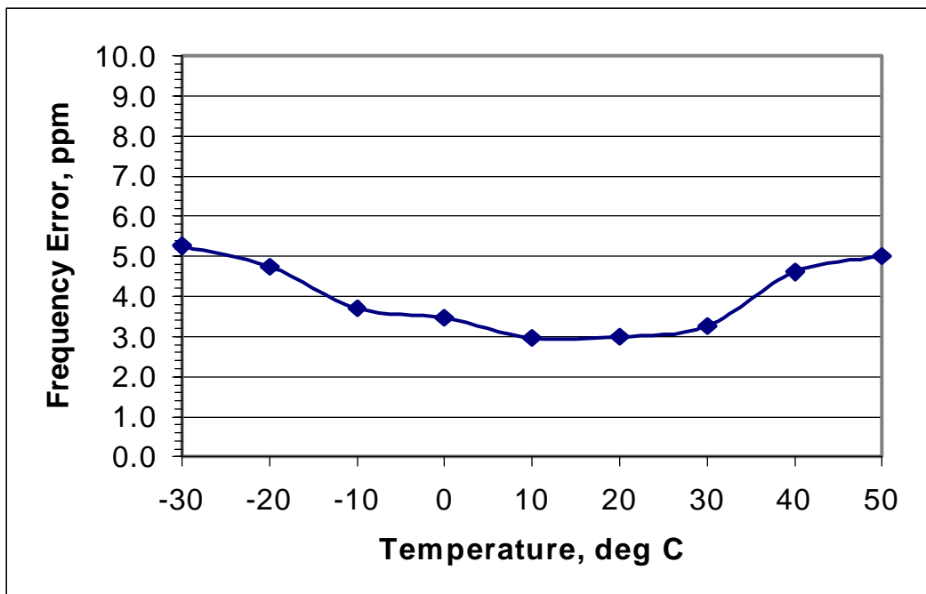
Exhibit 8 - RF Frequency Stability
