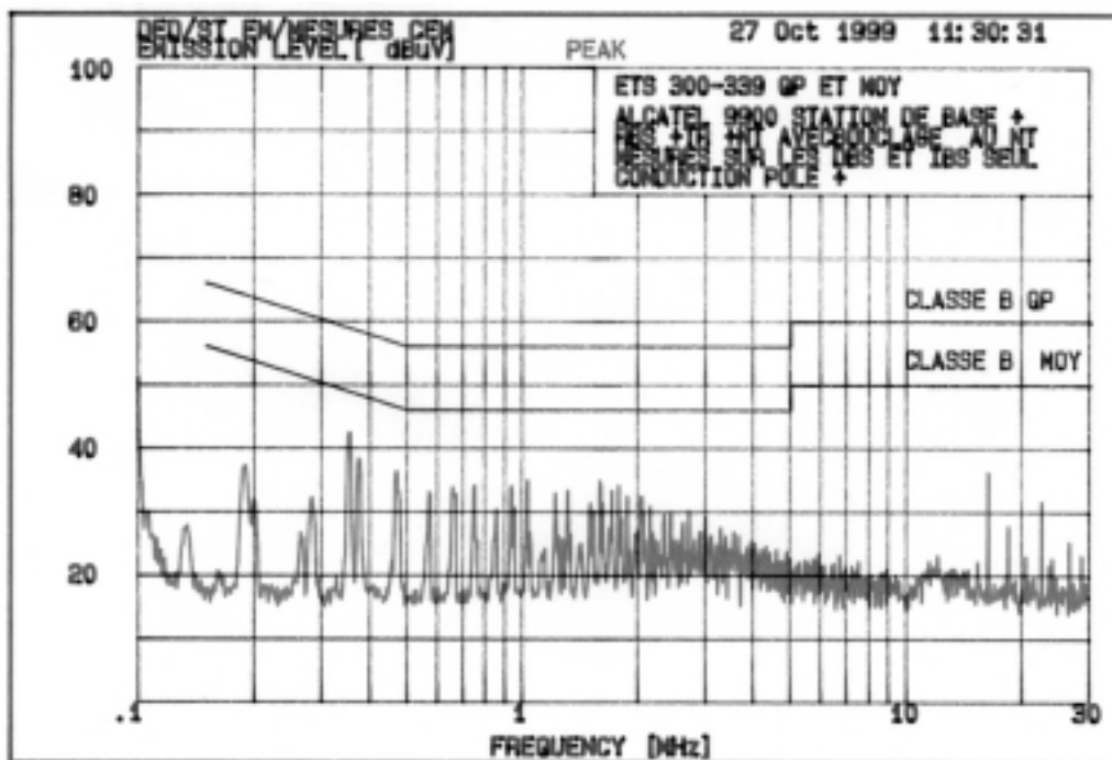
Exhibit 9 - Conducted Emissions on Positive Conductor
