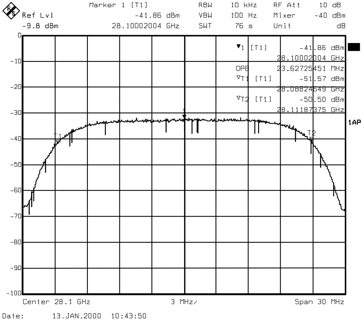
Exhibit 3 - Occupied Bandwidth
