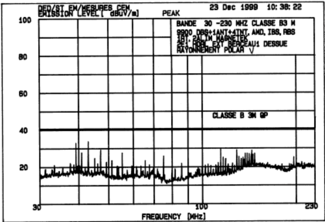
Exhibit 6 - Spurious Radiation (vertical)
