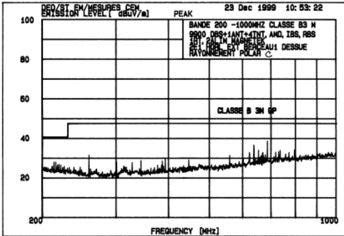
Exhibit 7 - Spurious Radiation (circular)
