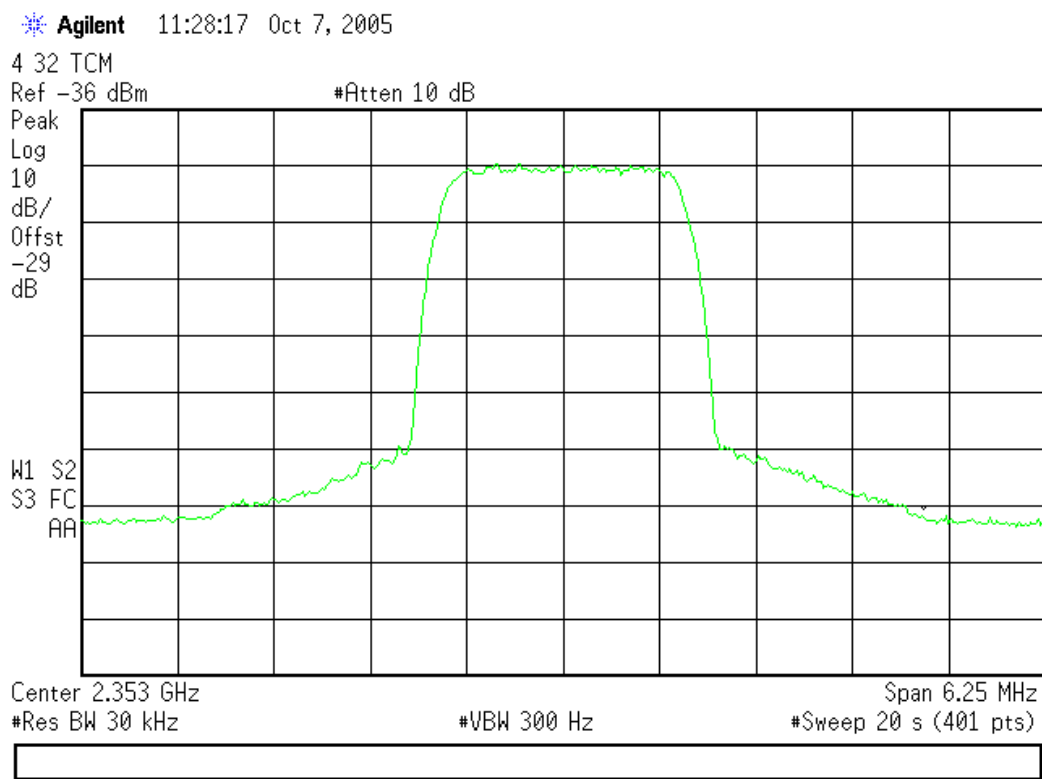
FIGURE 1. Typical Spectrum
