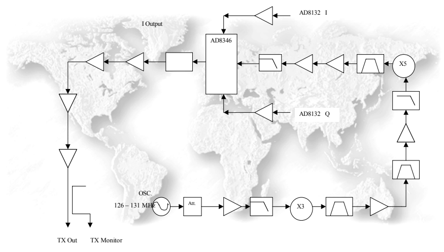
2 GHz RF TX Block Diagram
