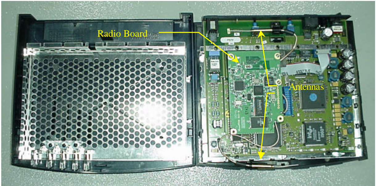
Figure 1 – Photo of EUT (with cover removed)
