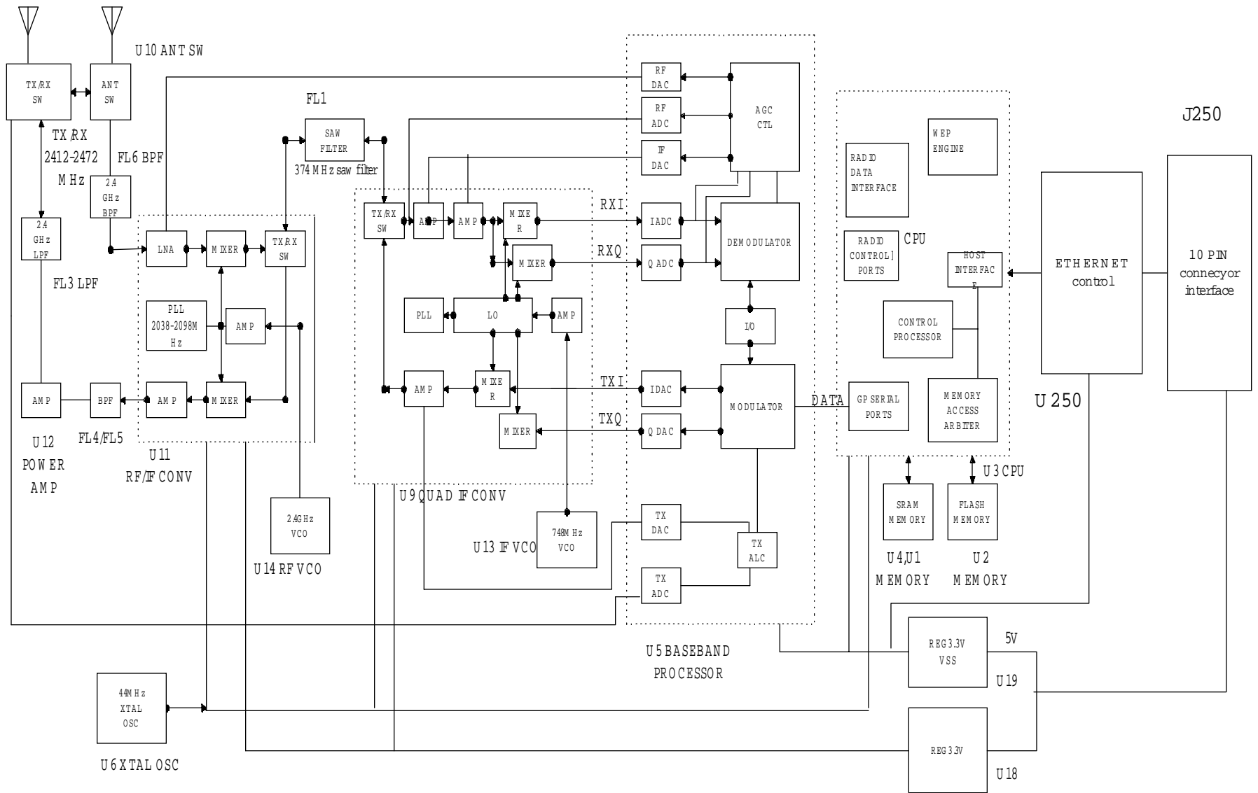
WX1513 BLOCKDIAGRAM
