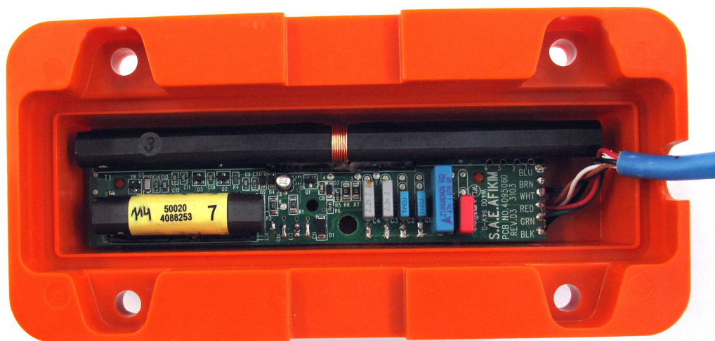
Photograph No 7 Antenna- Overall view
