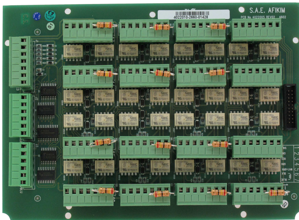
Photograph No.5 Switch box PCB view
