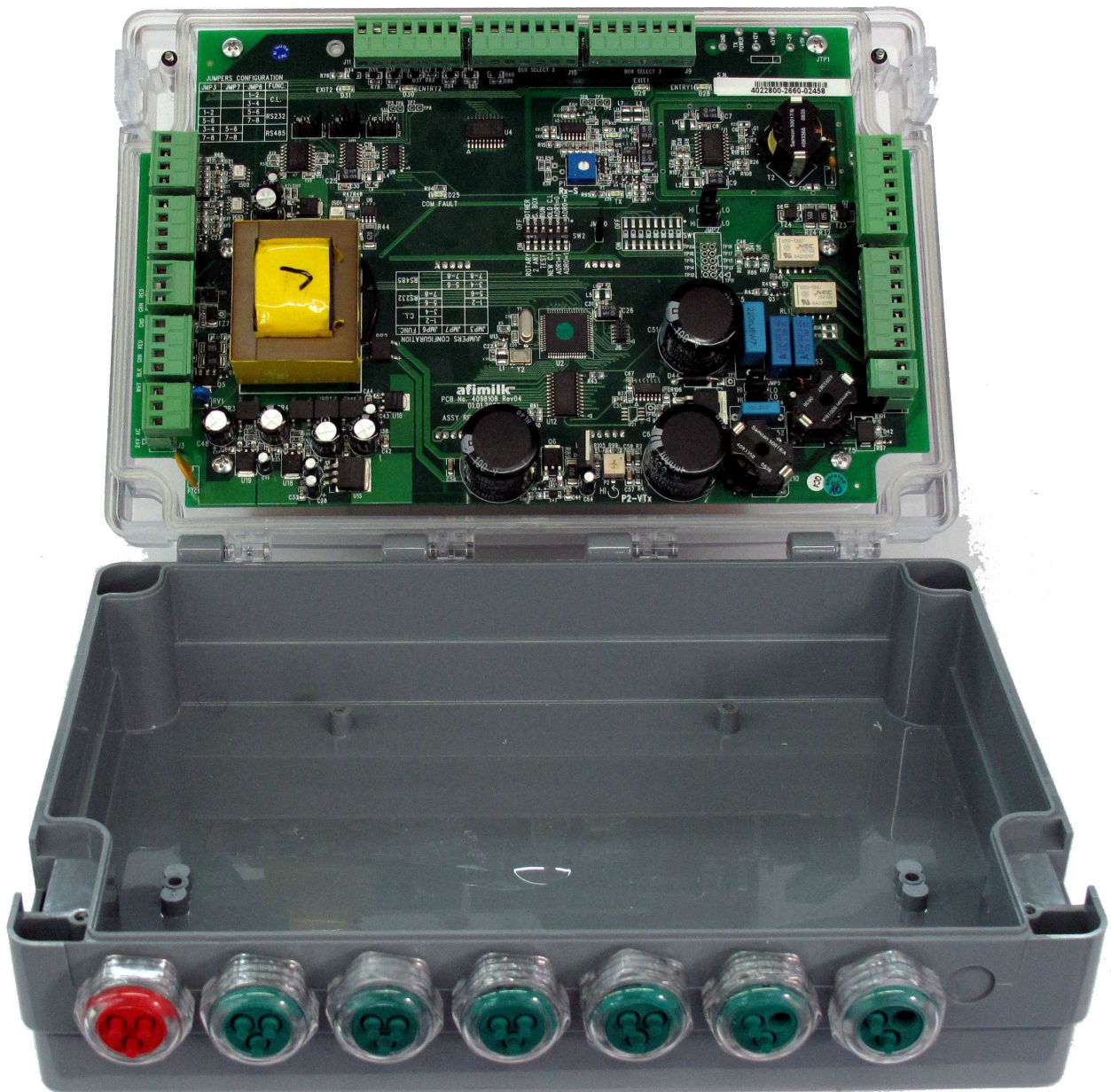
Photograph No.1 Ideal identification system controller internal view
