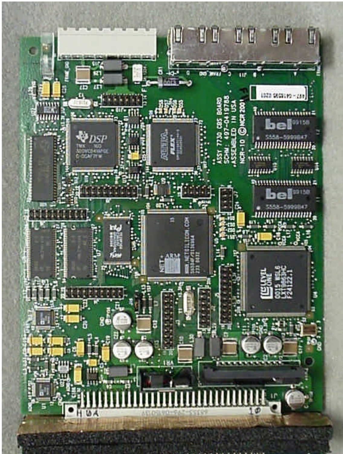
Photo 9. EUT, CBS Digital Board, Top View
