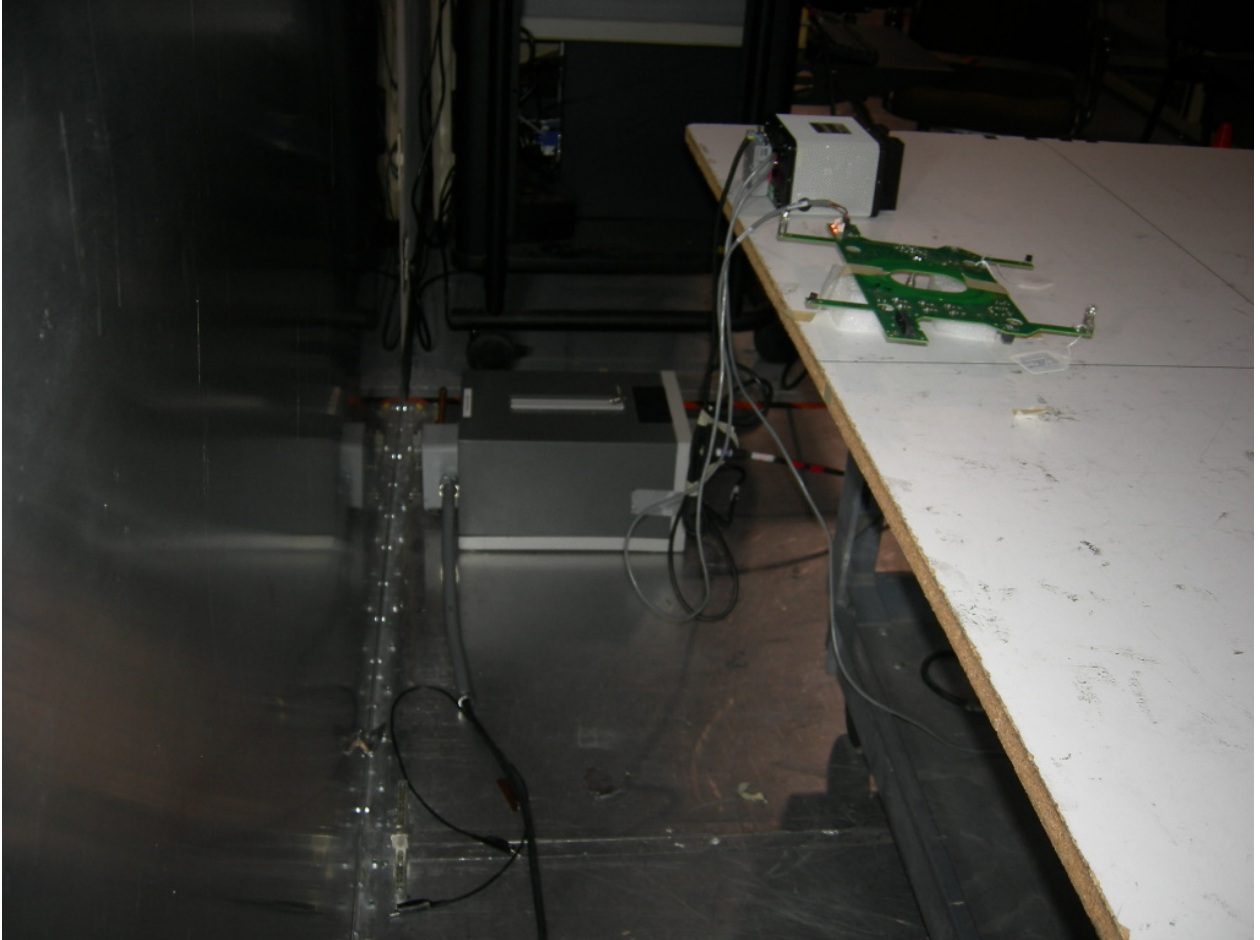
Figure 4: Conducted Emissions
