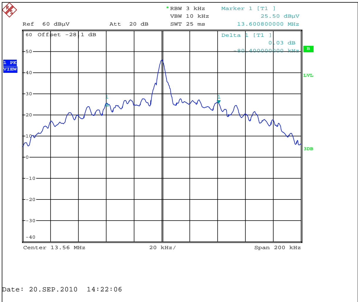
Figure 7.4.2-1: Occupied Bandwidth – 20dB
