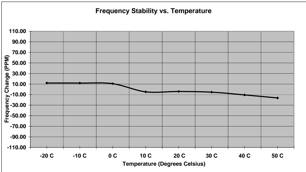
Figure 7.5.2-1: Frequency Stability
