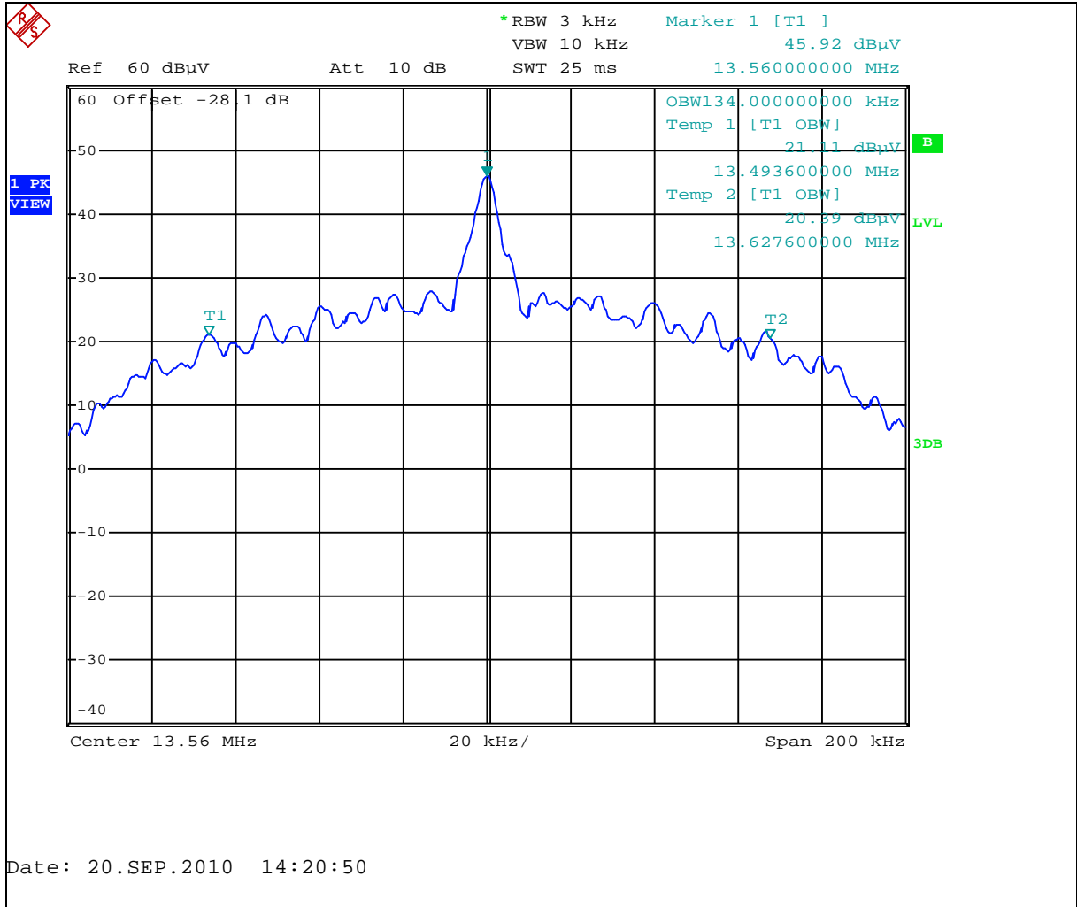
Figure 7.4.2-2: Occupied Bandwidth – 99%
