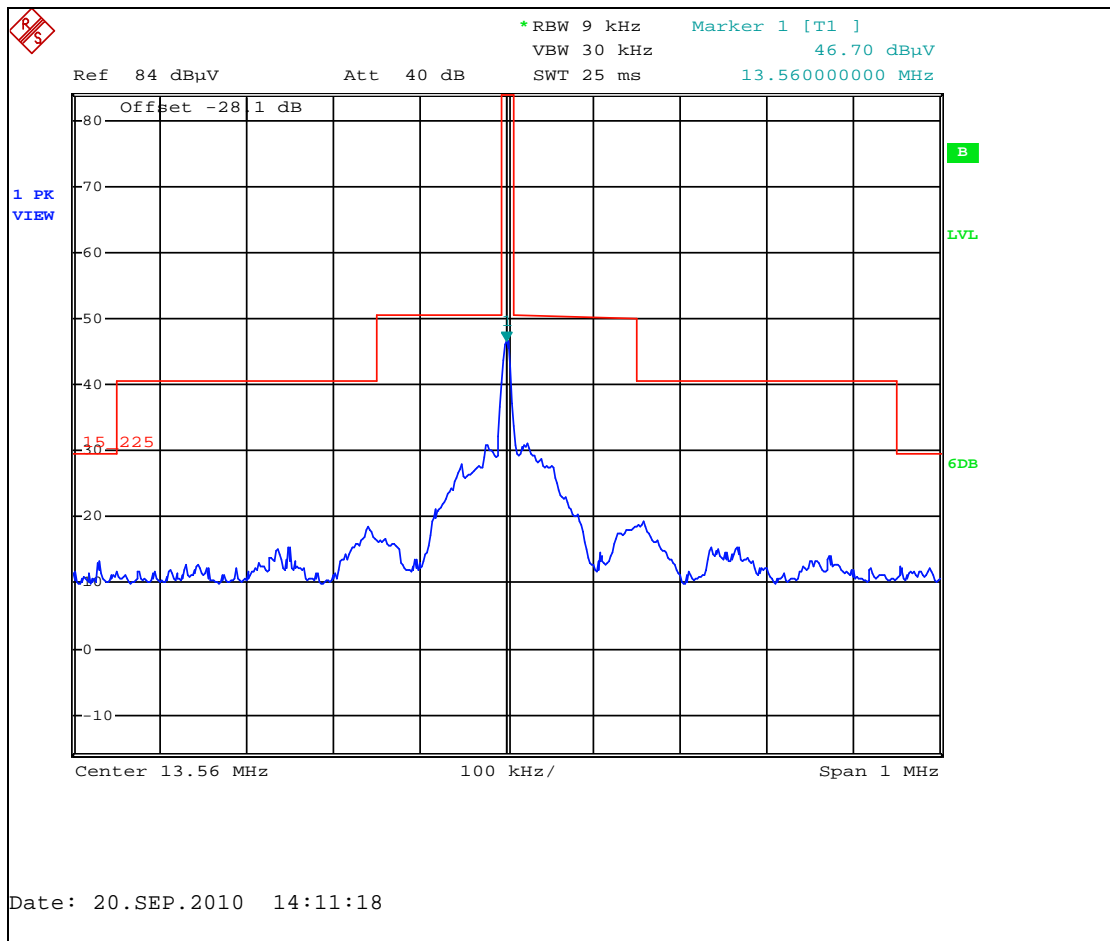
Figure 7.3.1-1: Emission Mask Plot
