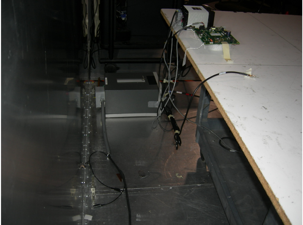
Figure 4: Conducted Emissions
