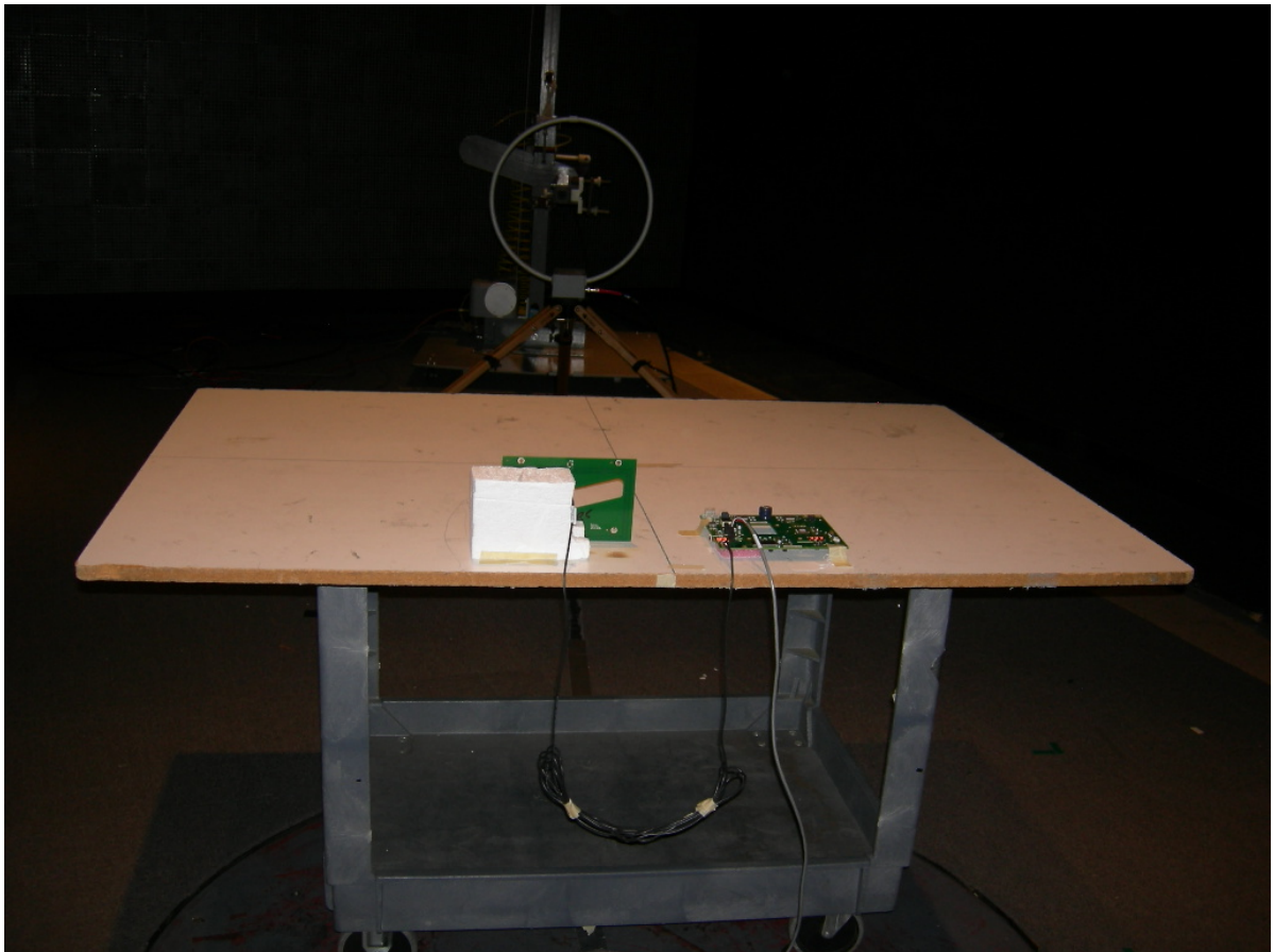
Figure 2: Radiated Emissions
