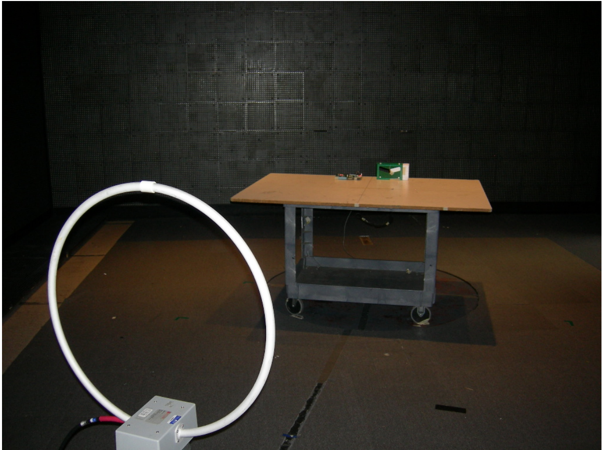
Figure 1: Radiated Emissions
