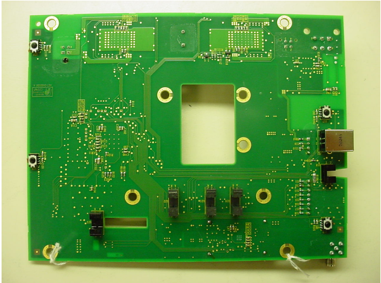
Figure 3: PCB - Back
