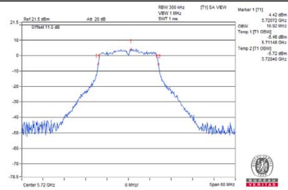
802.11ac (VHT20) / Chain 1 / CH 144
