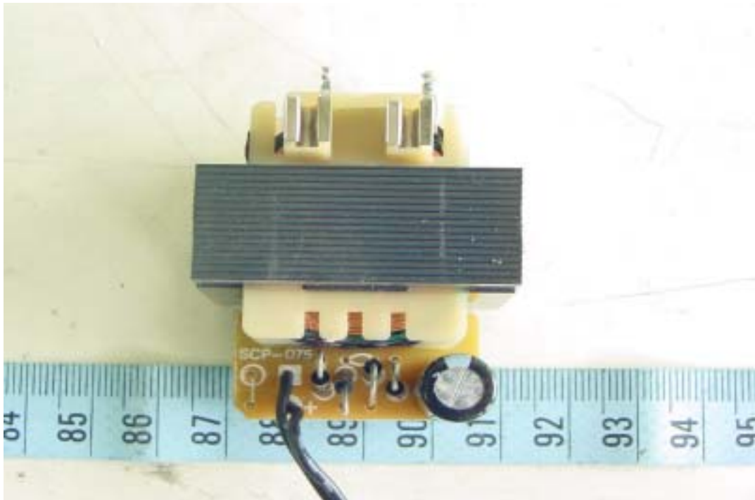
Component View of Adaptor's PCB
