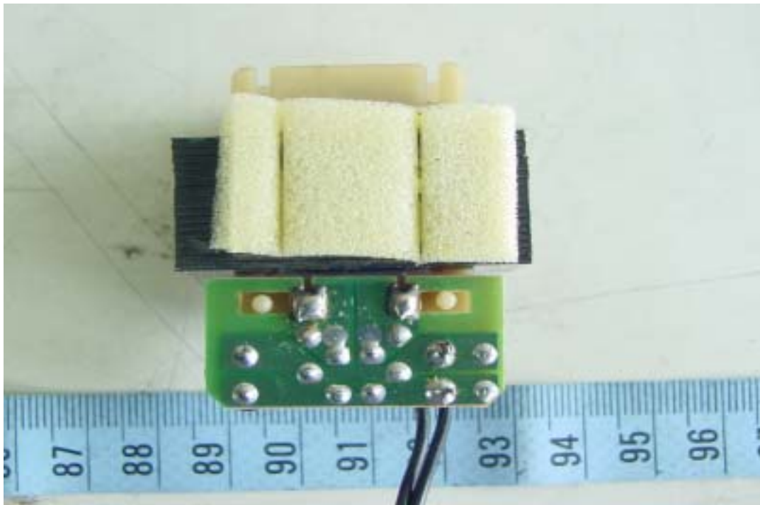
Solder View of Adaptor's PCB
