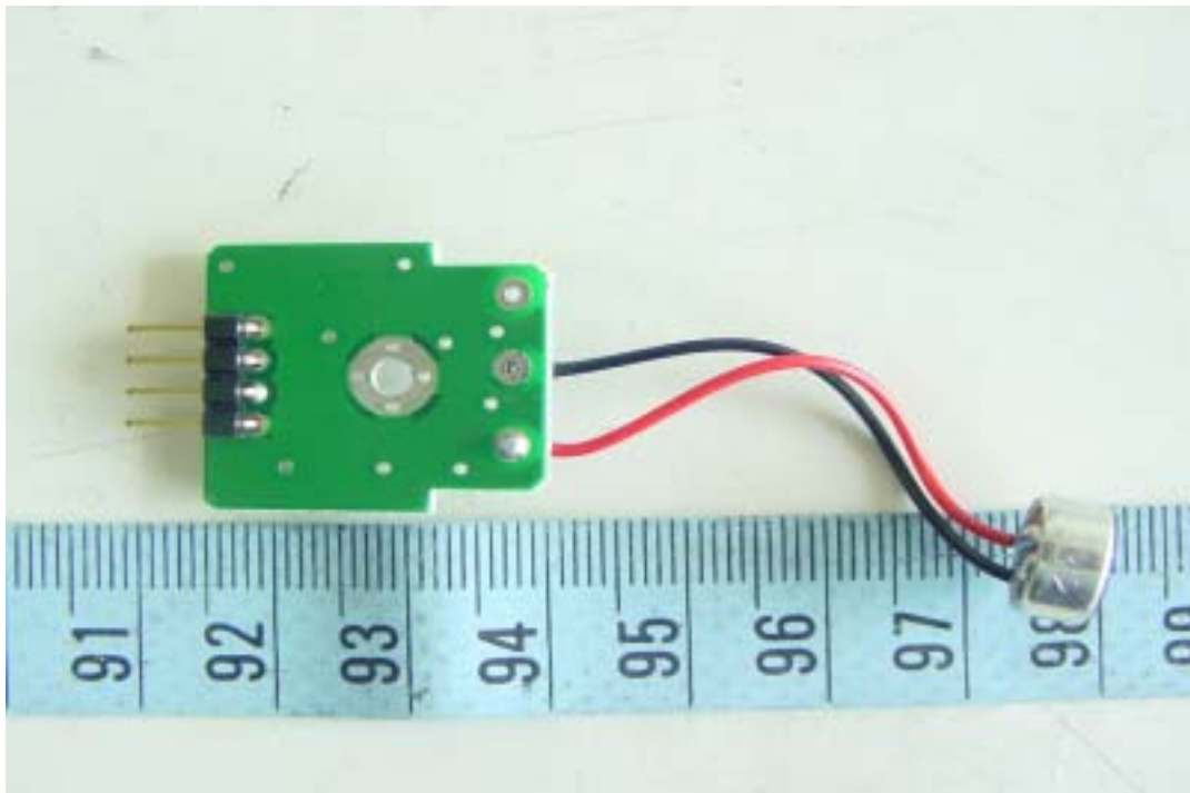
Solder View of Microphone PCB
