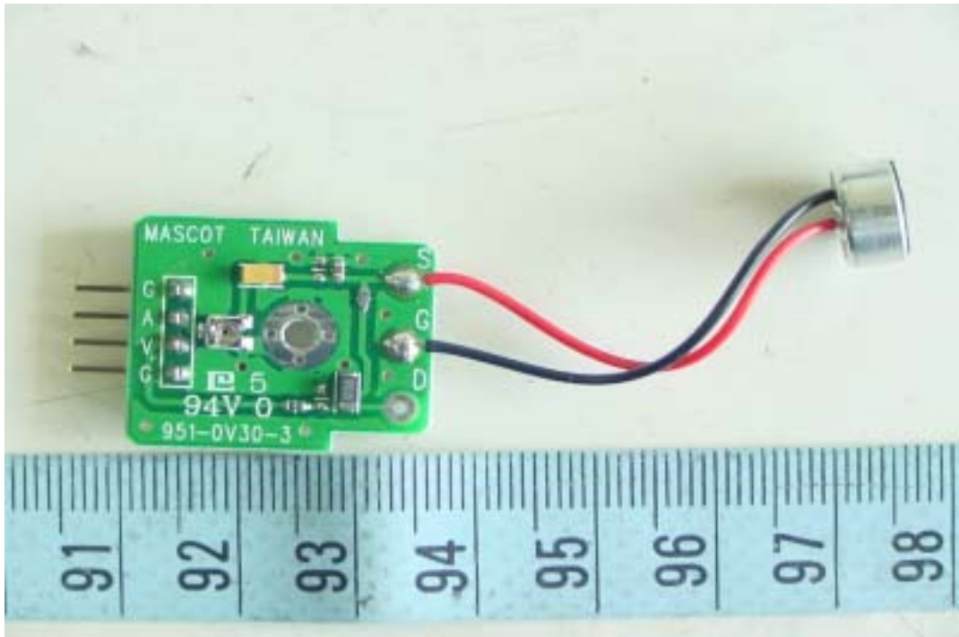
Component View of Microphone PCB
