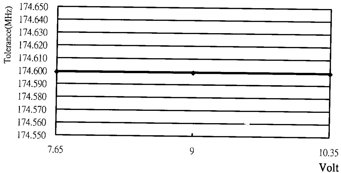
Voltage Variation Vs. Frequency Chart
