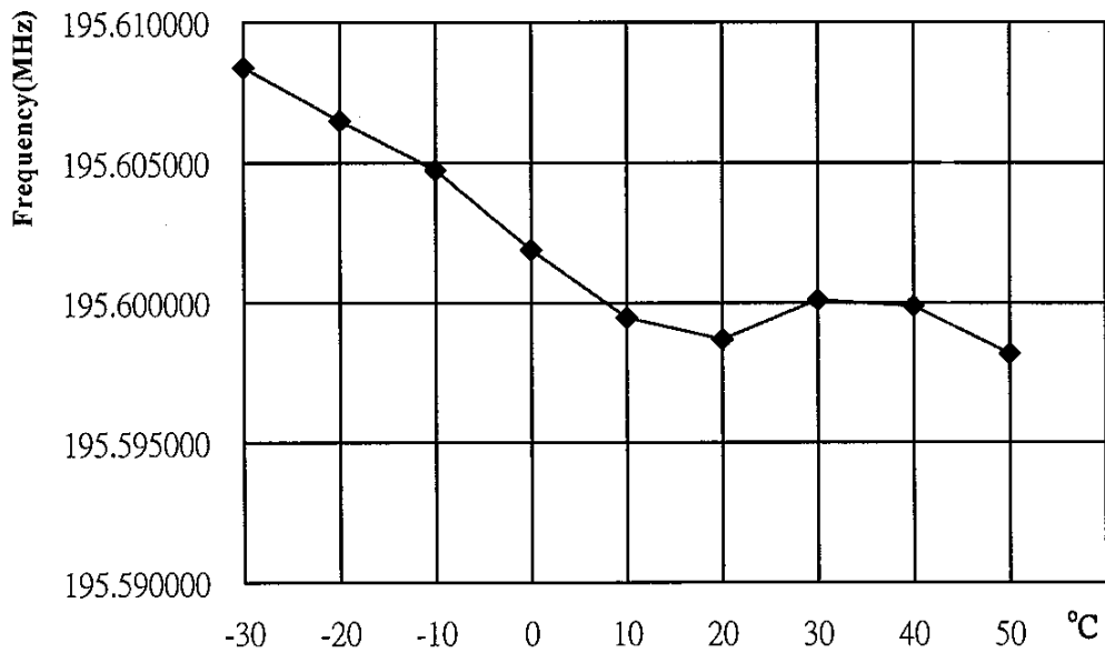
Temperature Variation Vs. Frequency Chart
