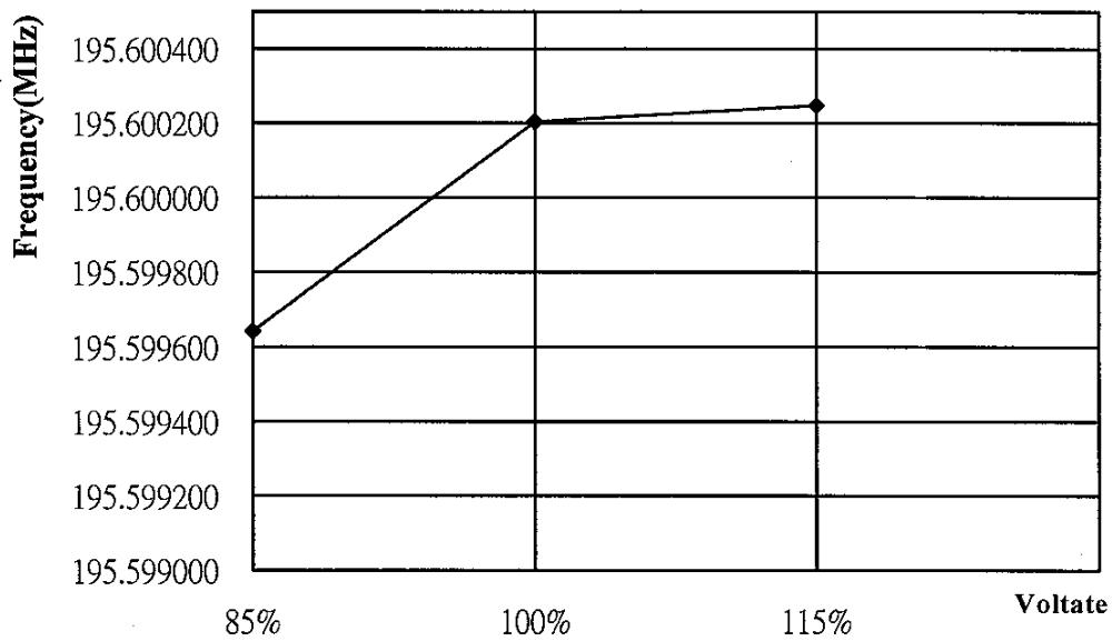
Voltage Variation Vs. Frequency Chart
