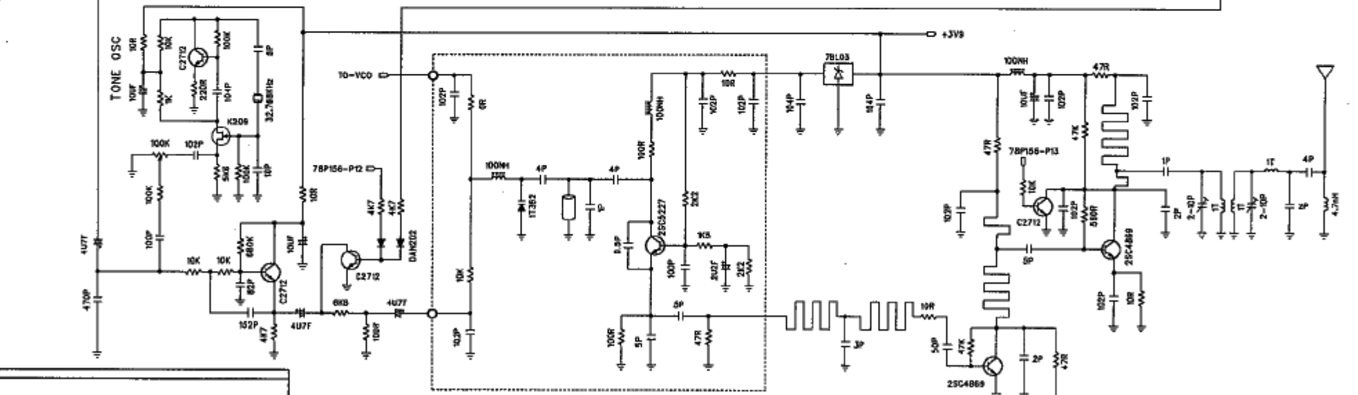
SCHEMATIC DIAGRAM UHF BAND PLL SYSTEM WIRELESS MICROPHONE MODEL : DX-837
