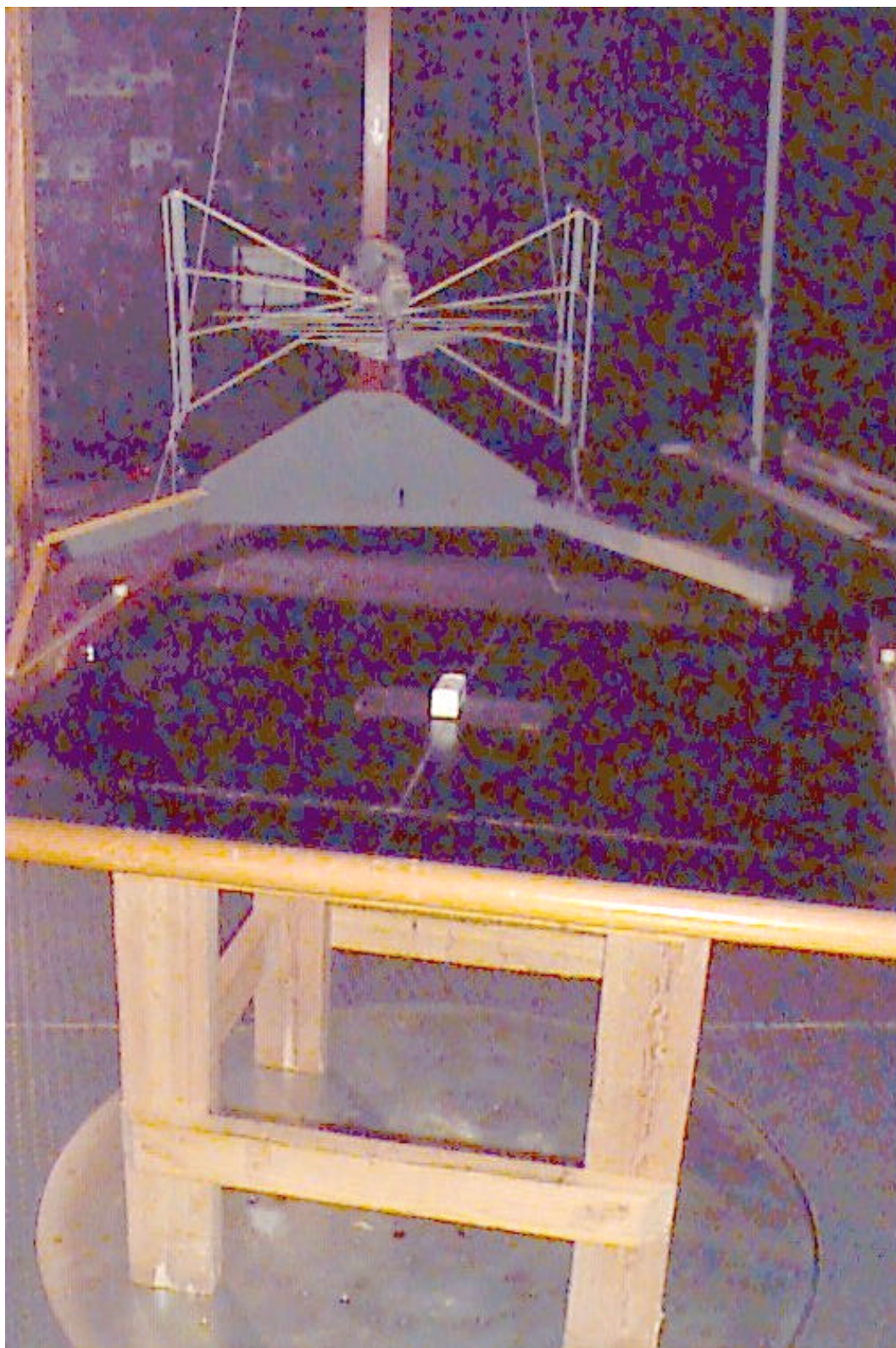
Photograph 1 Radiated emissions measurement test setup
