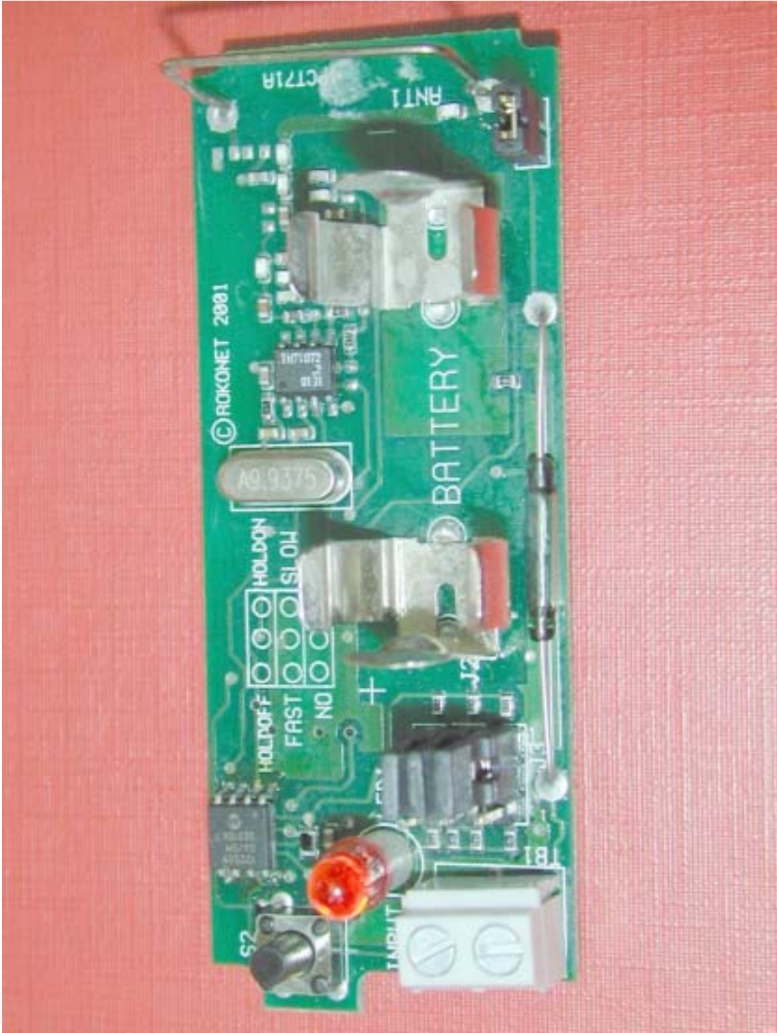
Photograph No.3 RWT71V2 detector PCB front view
