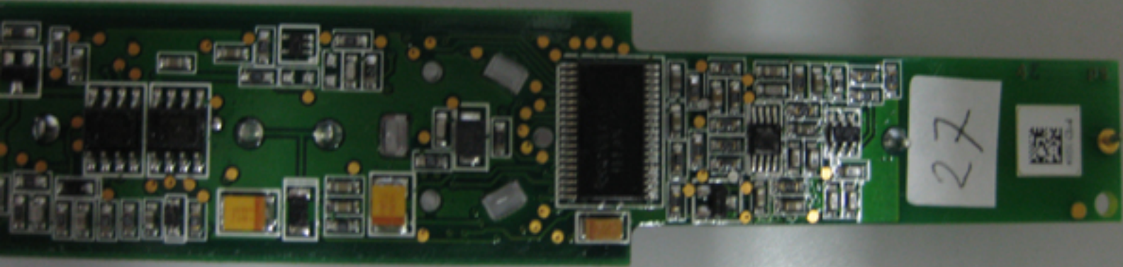
Transmitter Bottom Section 2
