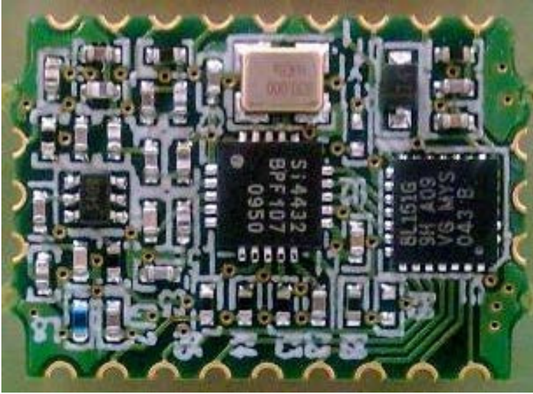
1. Photo of the 915Mhz stamp
