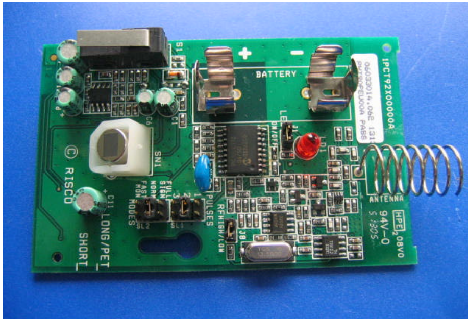
Photograph No.2 Component side of the main/RF PCB
