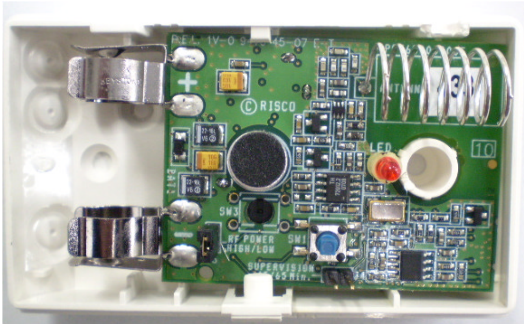
Photograph No.2 VITRON detector internal view with battery removed
