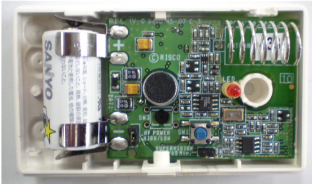
Photograph No.1 Wireless VITRON glass-break detector internal view
