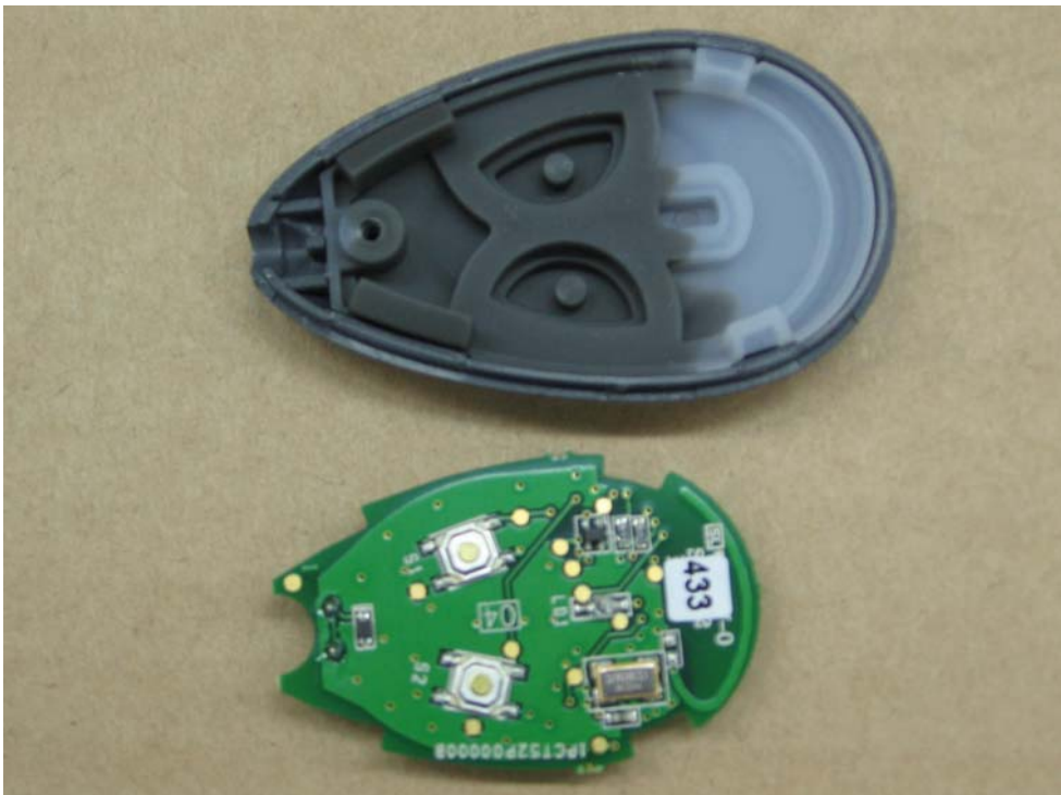
Figure 2: Top side of Unit
