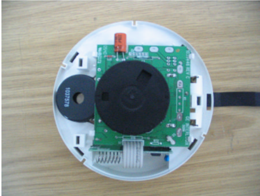
Photograph No.3 RWT30S433U SA detector internal view without the first internal cover
