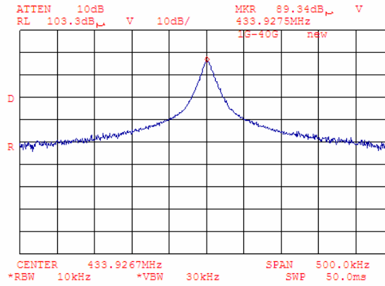
Plot 7.3.2 Occupied bandwidth test result
