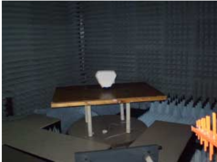
Photograph No.2 Radiated emission measurement test setup from 30 MHz to 1000 MHz
