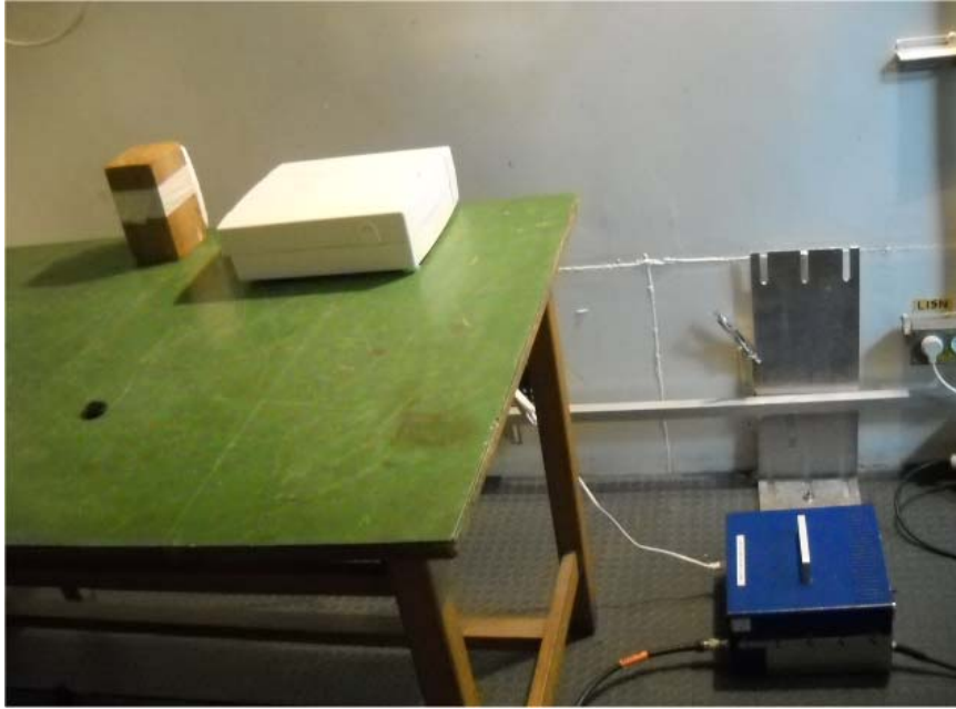
Photograph No.5 Setup for conducted emission measurements at the EUT power port
