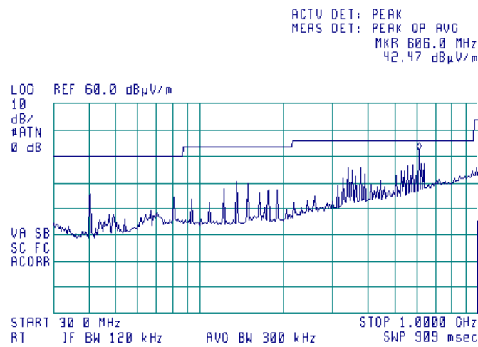
Plot 7.2.6 Radiated emission measurements from 30 to 1000 MHz
