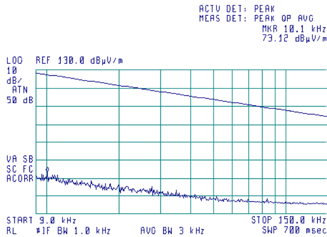
Plot 7.2.2 Radiated emission measurements from 9 to 150 kHz
