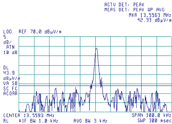
Plot 7.5.2 Occupied bandwidth test result high band edge
