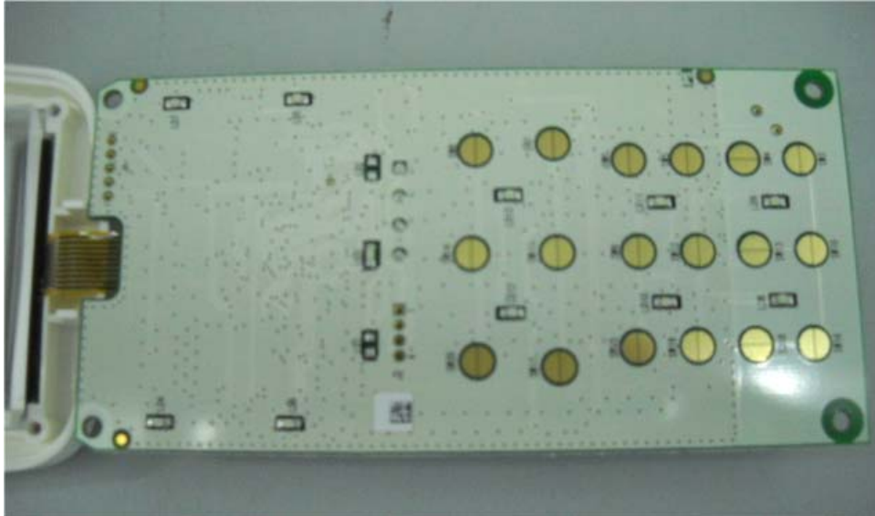
Photograph No.4 Keypad PCB second side view
