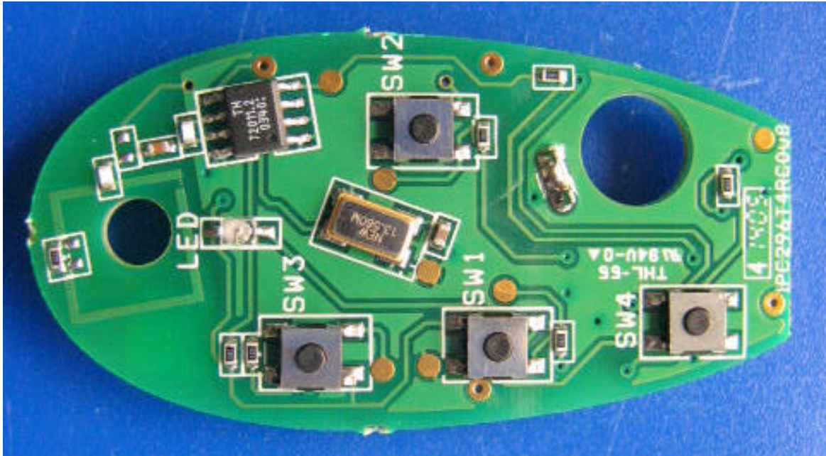
Photograph No.2 Component side of the main/RF PCB
