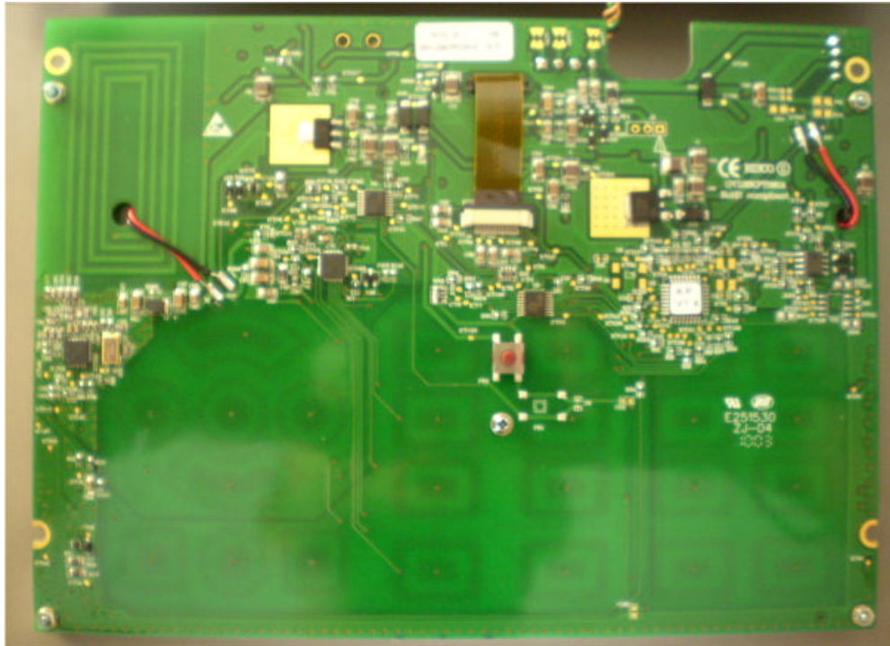
Photograph No.3 Touch screen keypad PCB second side view
