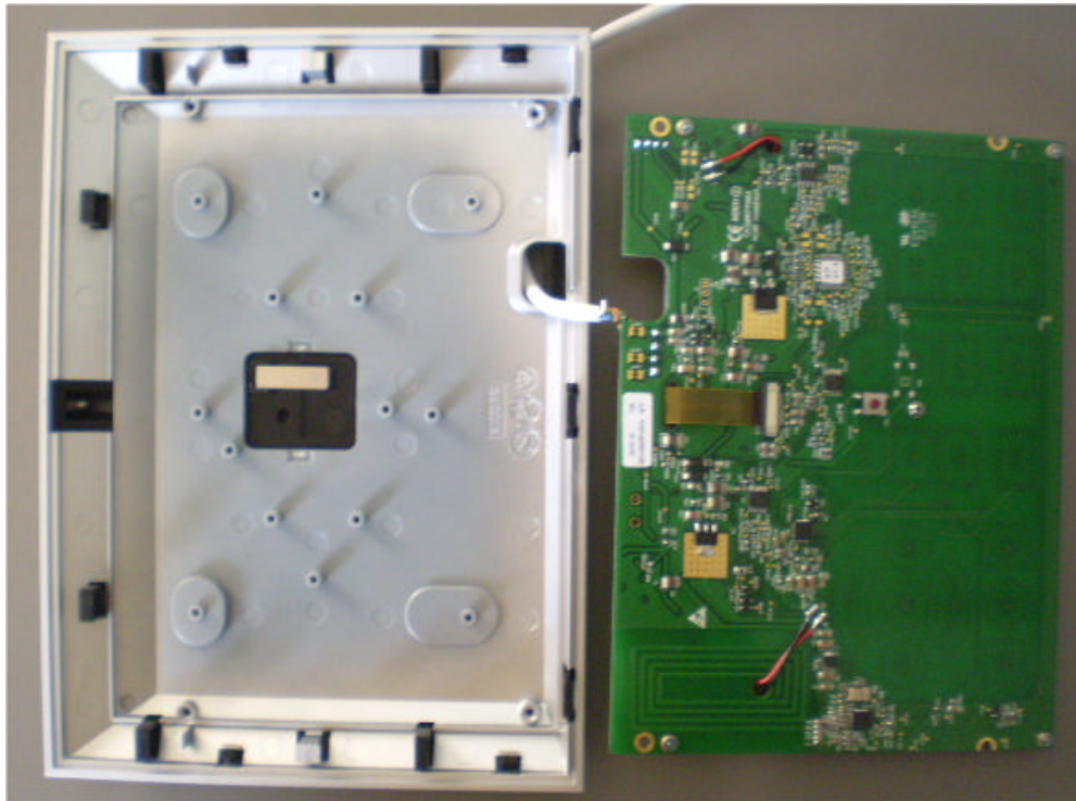
Photograph No.2 Touch screen keypad internal view
