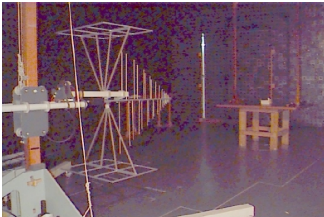
Photograph No.5 Radiated emission measurement test setup
