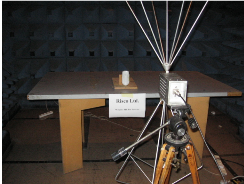
Figure 1. Radiated Emission Screening Test, Host: Two Way Wireless PIR Detector
