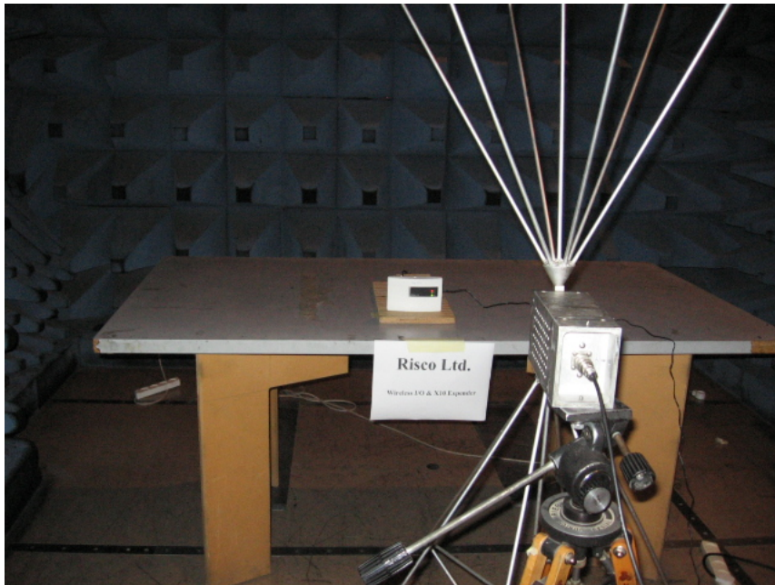
Figure 3. Radiated Emission Screening Test, Host: Two Way I/O Expander
