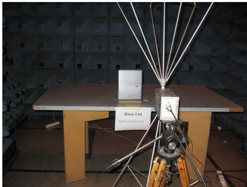
Figure 2. Radiated Emission Screening Test, Host: Agility Control Panel
