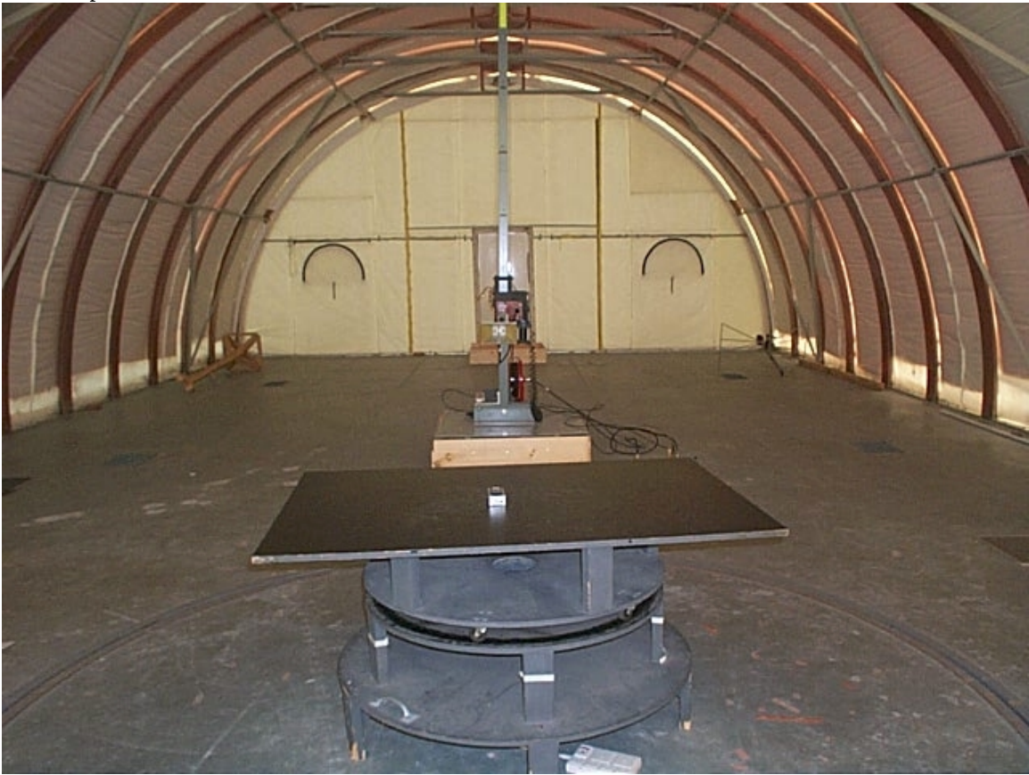
Test Setup Back
