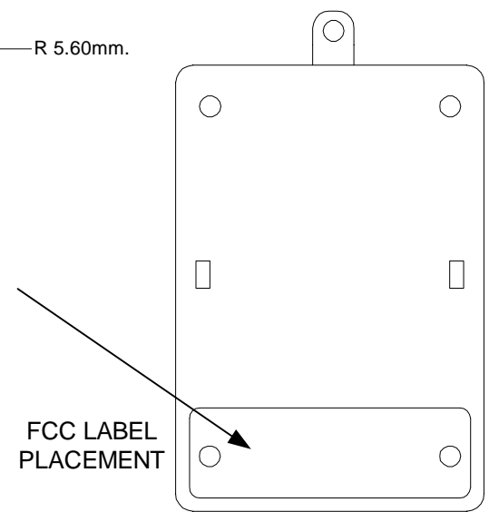
BOTTOM VIEW OF THE PLASTIC CASE
