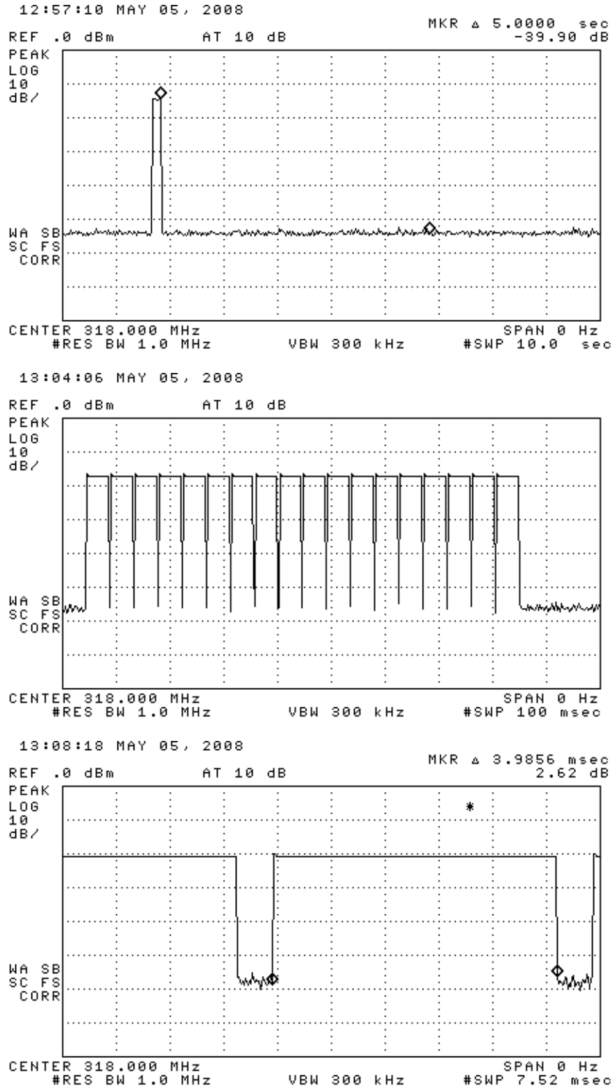
Figure 6.1(a). Transmission modulation characteristics. (top) single button press, (center) expanded transmission, (bottom) expanded bit(s).
