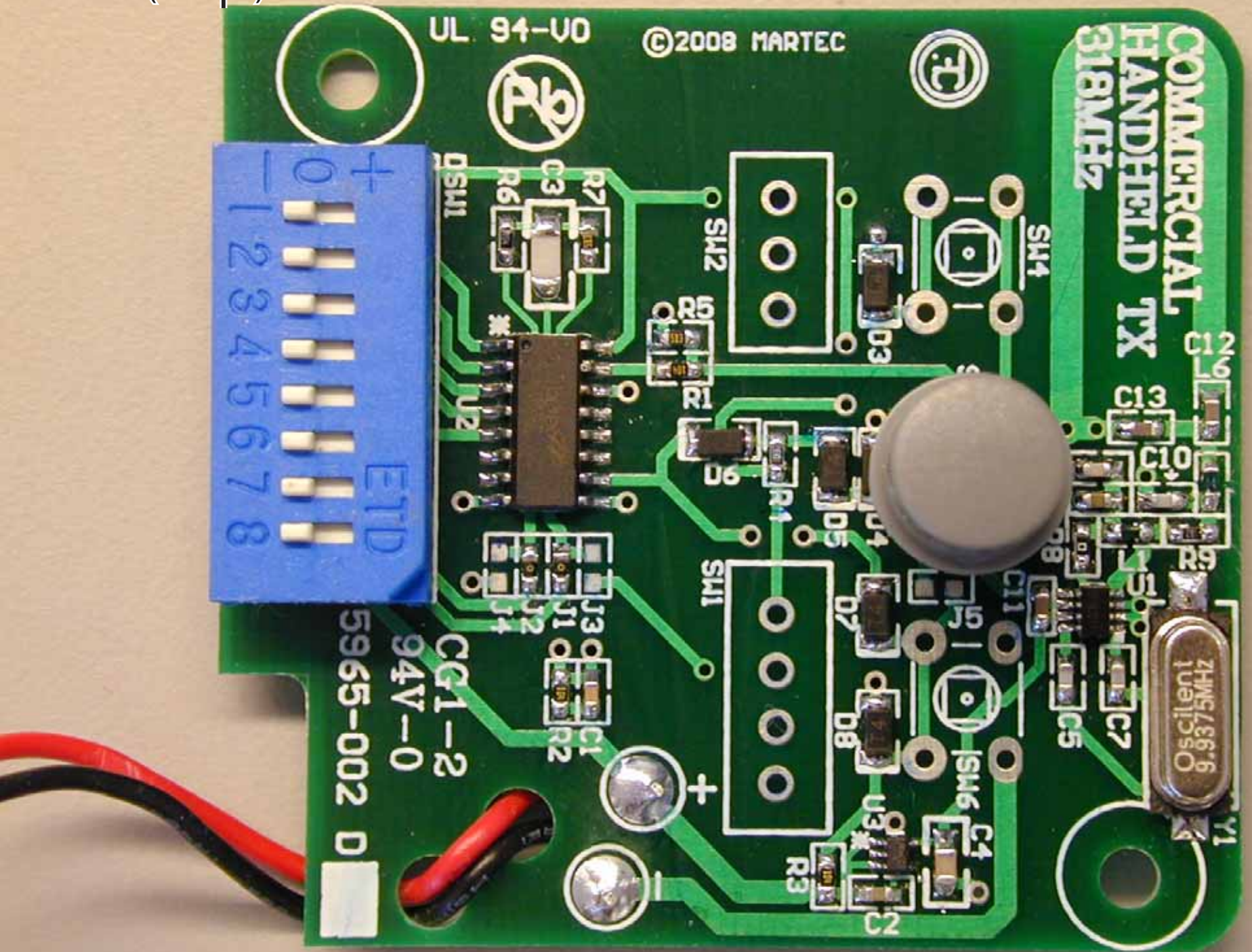
PCB (top)
