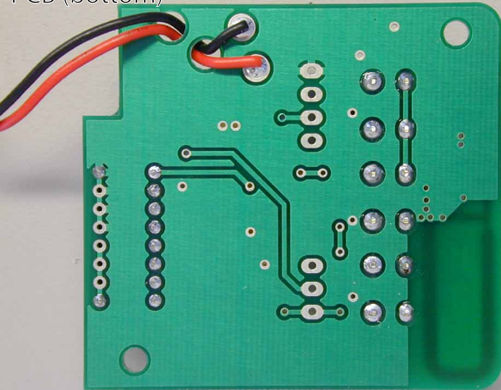
PCB (bottom)
