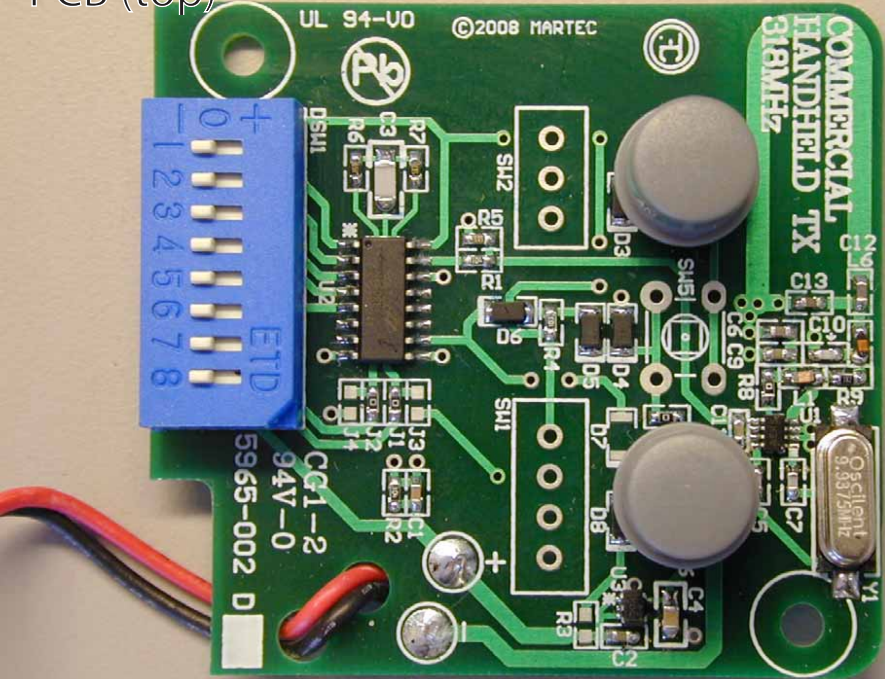
PCB (top)
