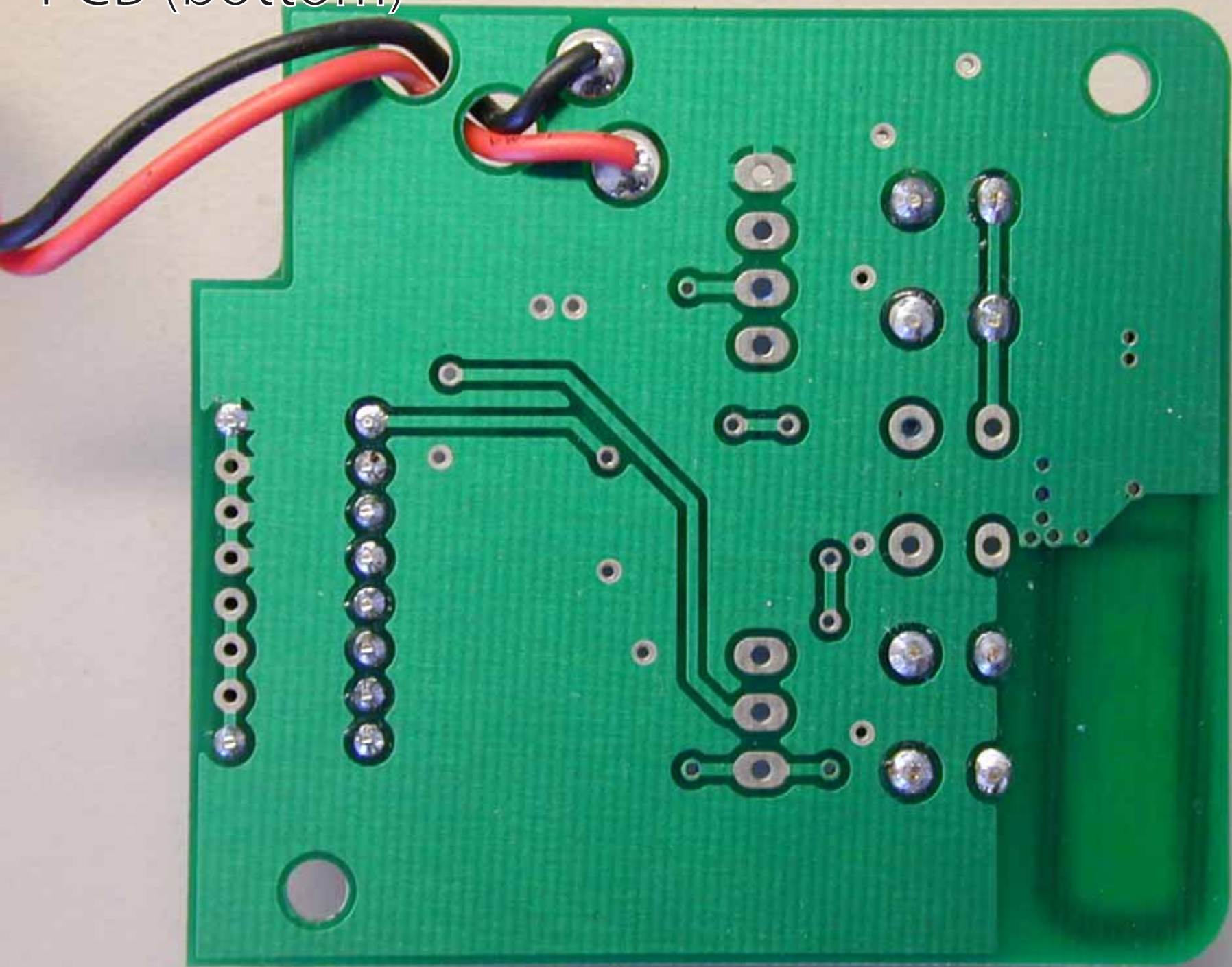
PCB (bottom)
