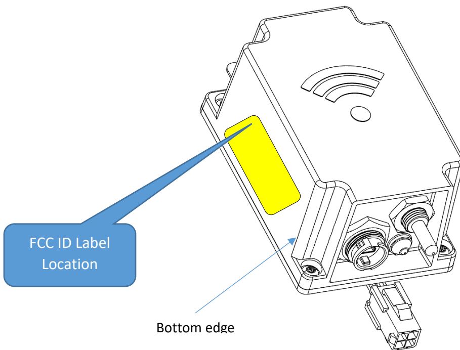
Figure 1: Wireless Monitor showing FCC label optional locations (blank)
